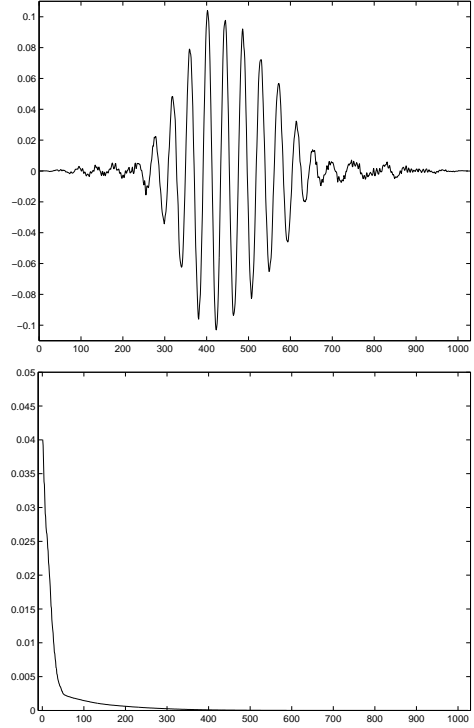
Figure 2: The first principal component (upper graph) and the eigen-value profile (lower graph) of phoneme IY.
