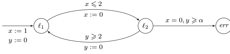
(a) A timed automaton \mathcal{A}_\alpha .
