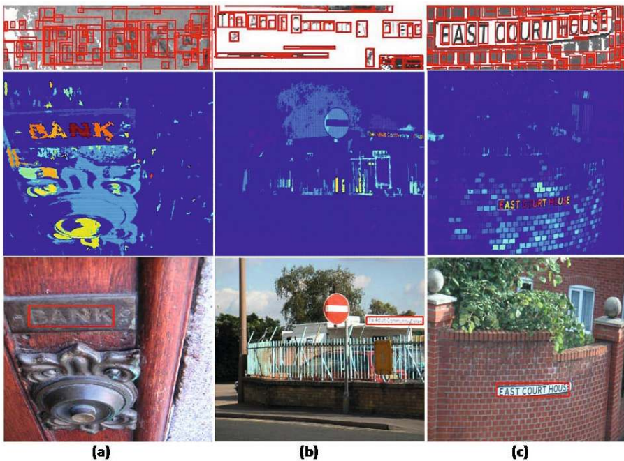
Fig. 2. The performance of the MSERs detector and the CNN classifier for low contrast (a) and low quality texts (b), and text-like outliers (c). The top row are the MESERs detections on text areas. The middle row are the confident maps generated by the CNN classifier. The pixels are displayed by their higher confident scores if they belong to multiple components. The bottom row are the detection results.
