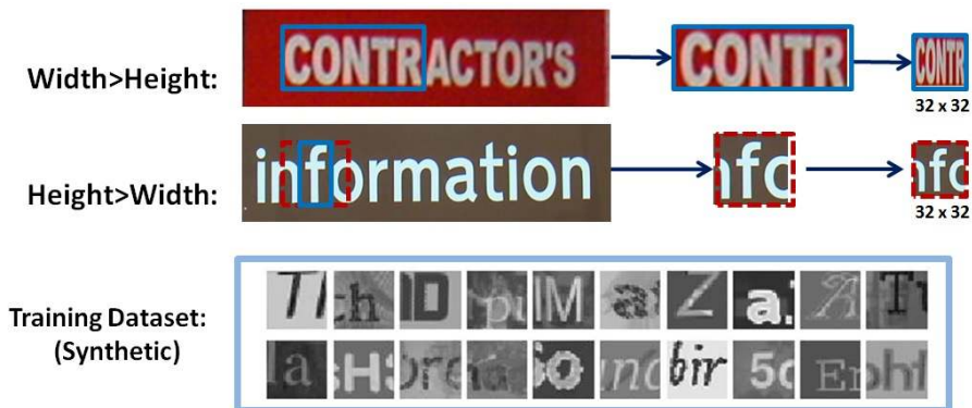
Fig. 3. MSERs component alignment with size of 32 \times 32 and synthetic training samples
