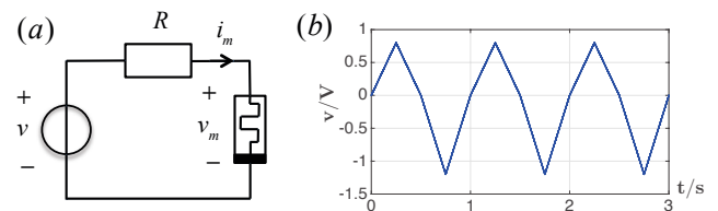
Fig. 5. (a) Test circuit with series resistor. (b) Time waveform of the asymmetric triangular voltage waveform of period T = 1 s driving the circuit in plot (a).
