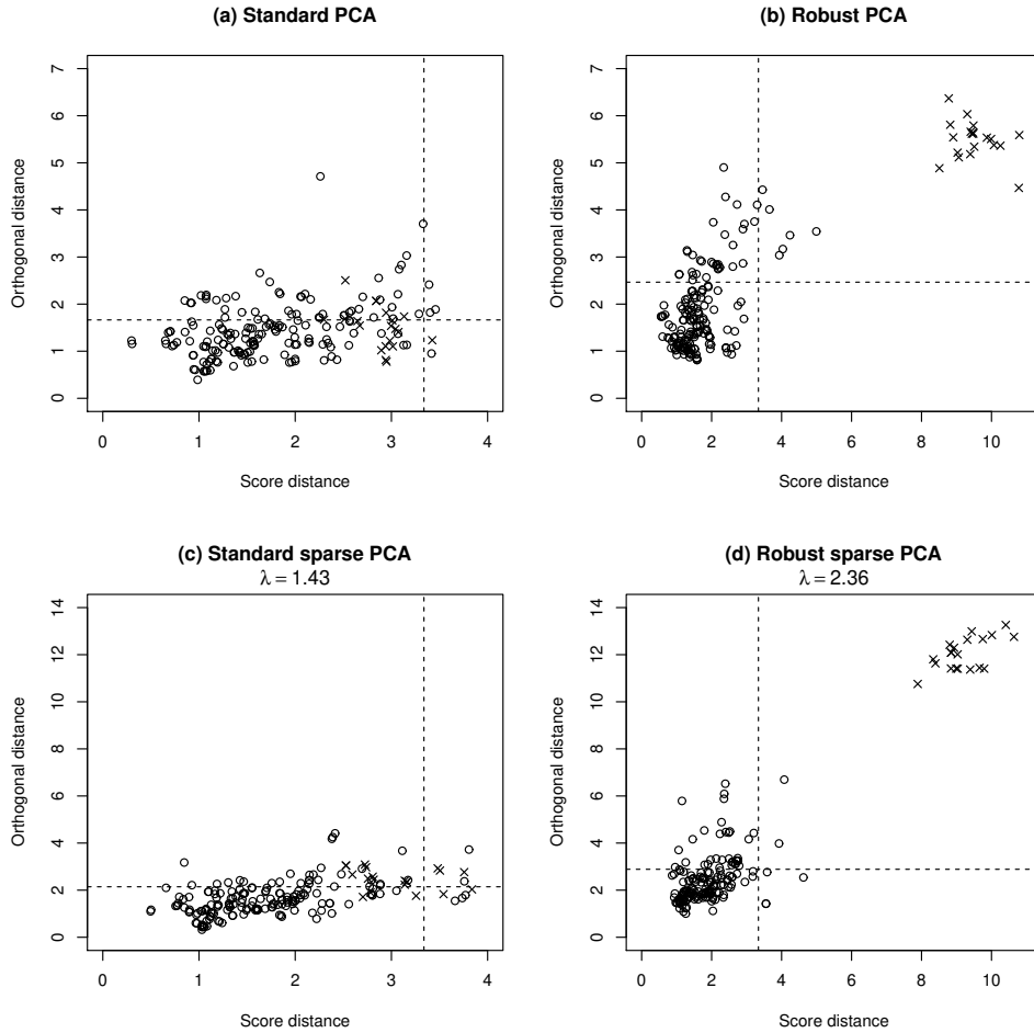
Figure 4: Distance-distance plots for standard and robust PCA and their sparse versions. In the robust plots vehicles running on diesel ( \times ) are clearly distinguishable from vehicles using gasoline ( \circ ).
