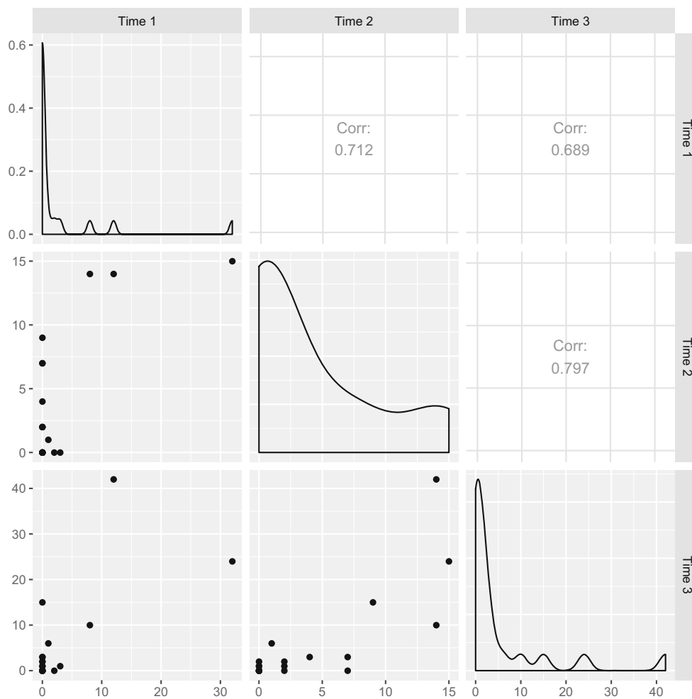
Fig. 1 Scatterplot matrix for hangover data. The upper triangle panels report the Pearson correlations
