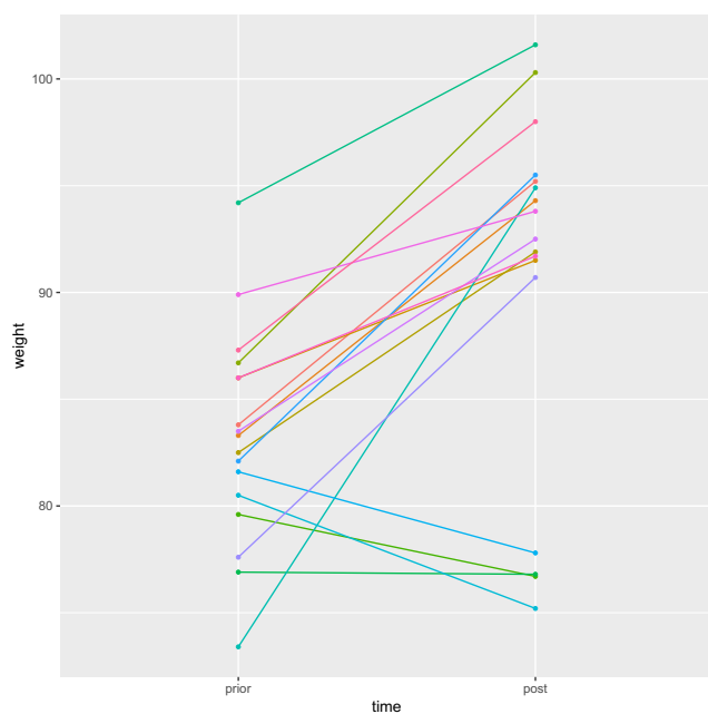
Fig. 3 Individual weight trajectories of anorexic girls before and after treatment
