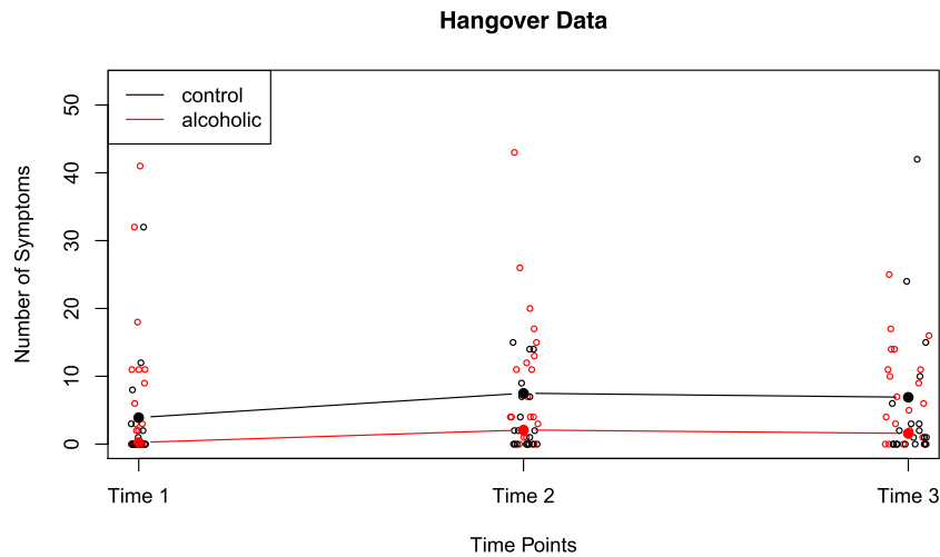
Fig. 7 20% trimmed means of the number of hangover symptoms across three time points
