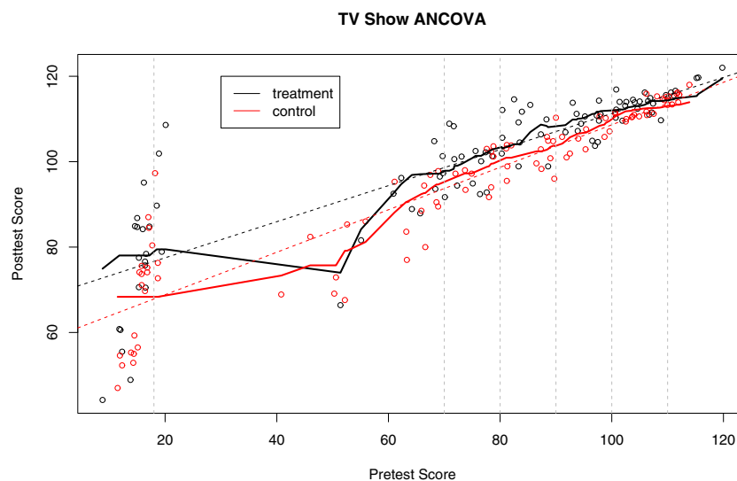
Fig. 9 Robust ANCOVA fit on TV show data across treatment and control group. The nonparametric regression lines for both subgroups are shown as well as the OLS fit ( dashed lines ). The vertical lines show the design points our comparisons are based on
