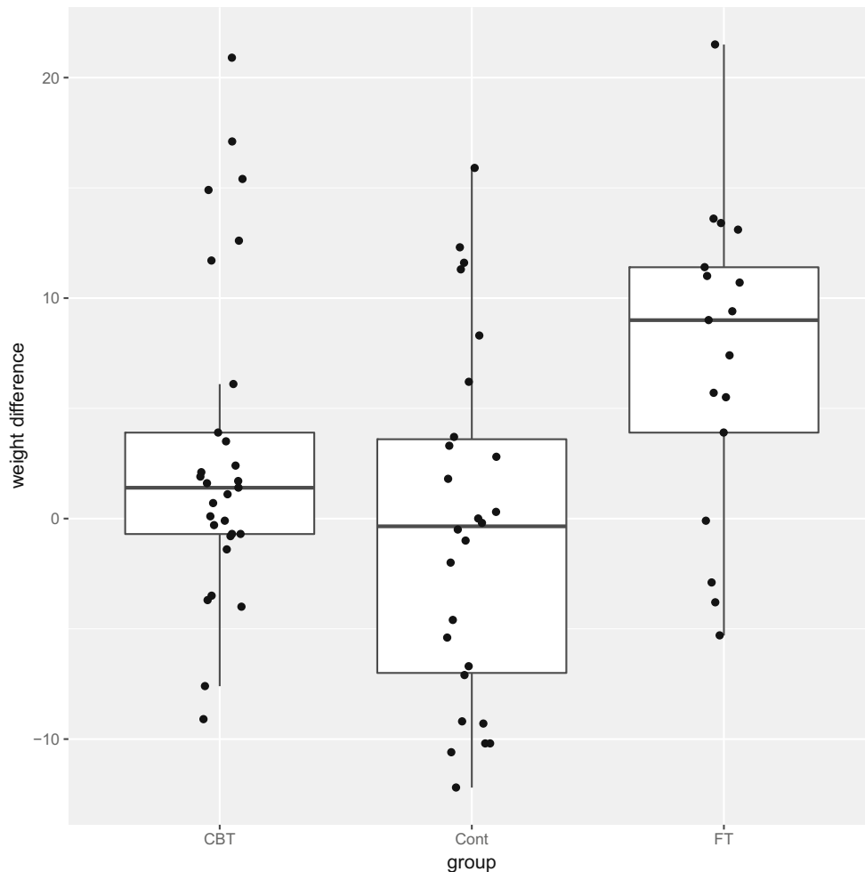
Fig. 4 Boxplots with superimposed jittered 1D scatterplots for weight differences across control and two treatment conditions
