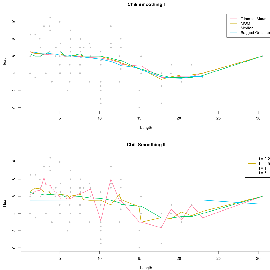
Fig. 8 Top panel: smoothers with various robust location measures. Bottom panel: trimmed mean smoother with varying smoothing parameter f
