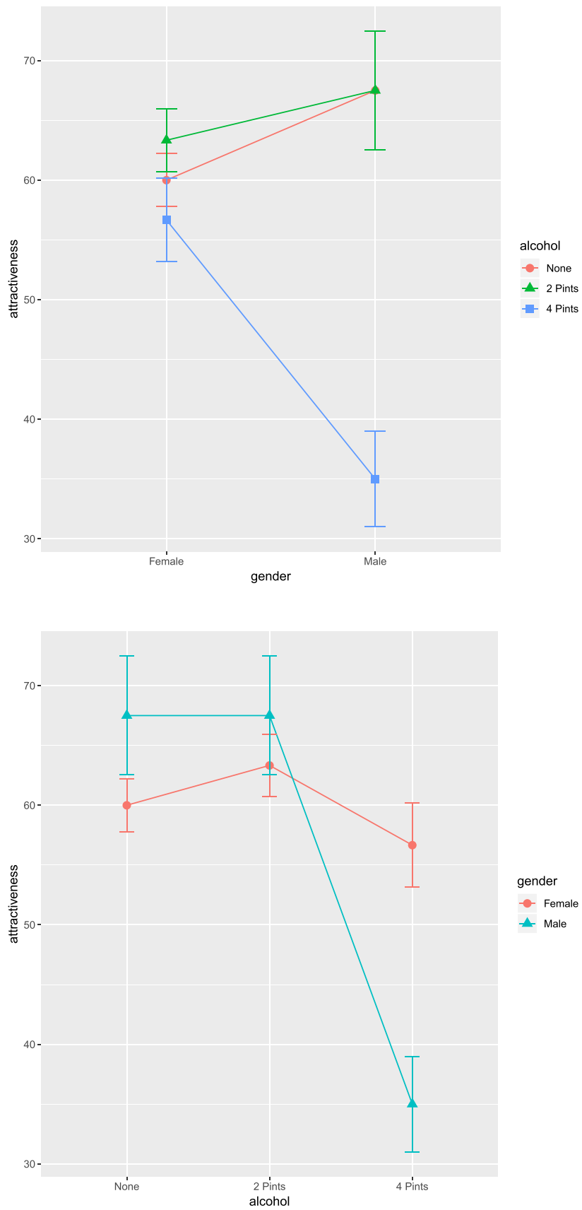
Fig. 5 Trimmed means interaction plots for beer goggles dataset
