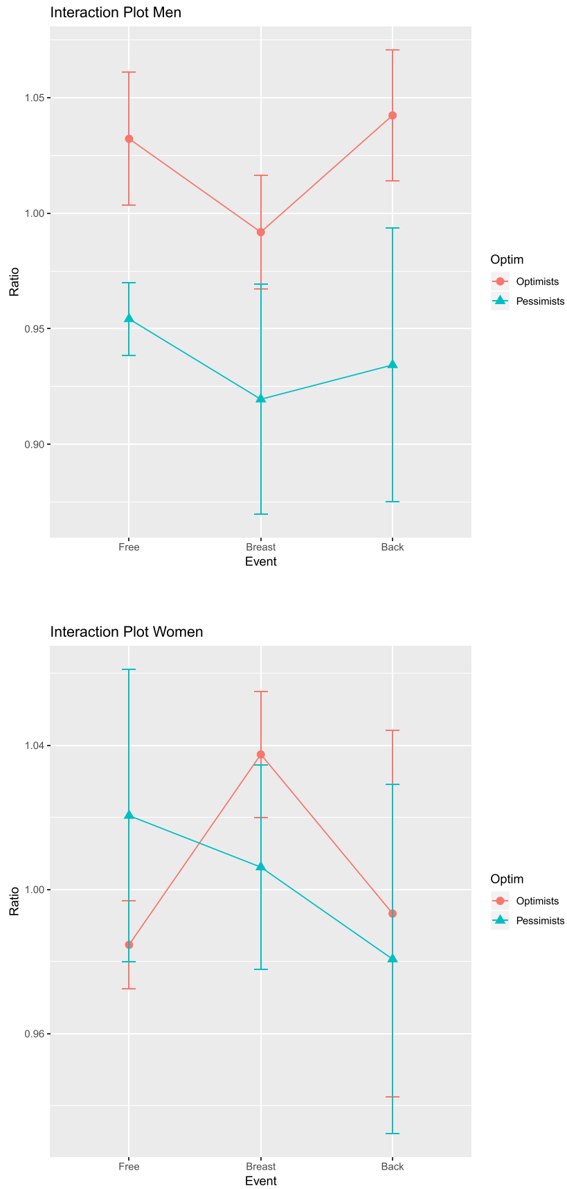
Fig. 6 Interaction plot for the trimmed means of the time ratio response for males and females separately
