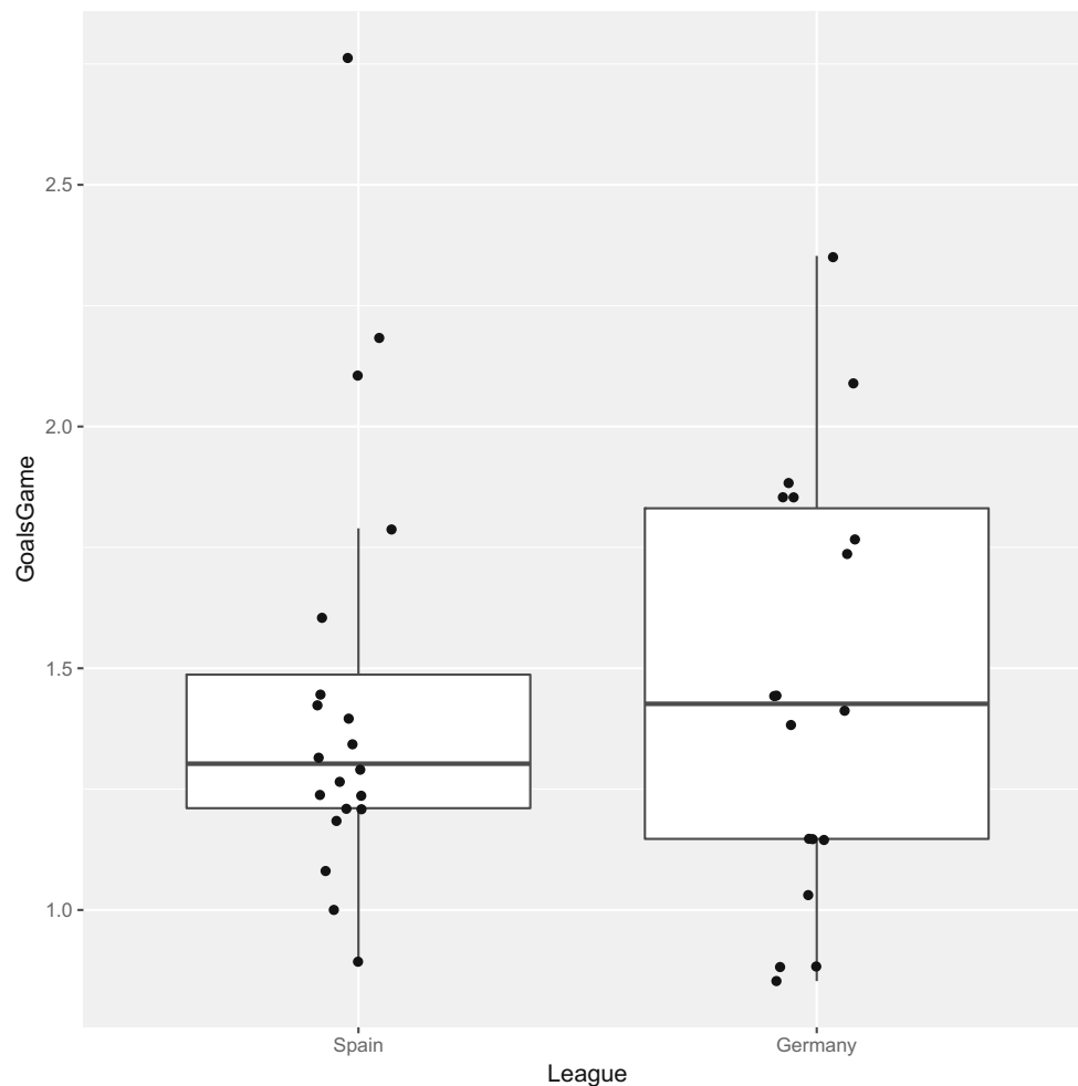
Fig. 2 Boxplots for scored goals per game (Spanish vs. German league) with superimposed 1D jittered scatterplot
