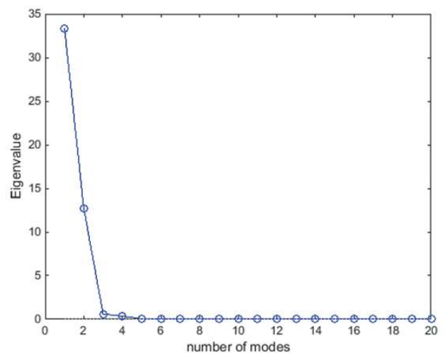
Fig. 2 Correlation eigenvalues of random field Z
