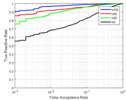
Fig. 4. Different number of training image sets and their ROC curves
