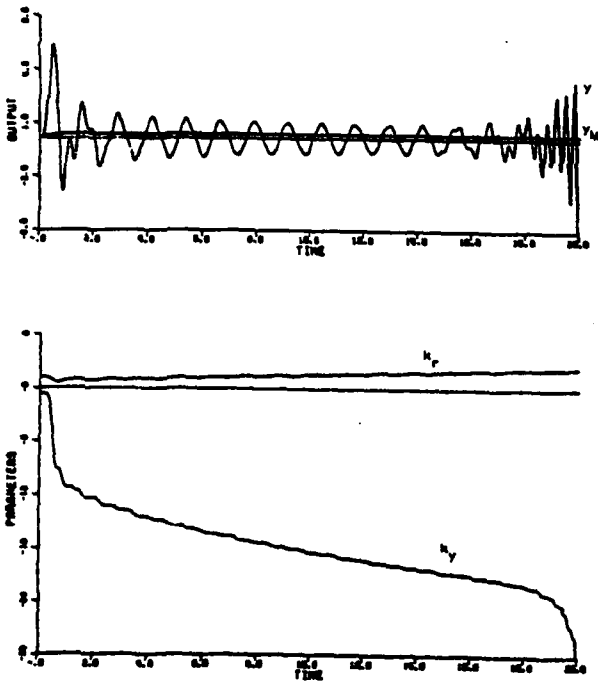
Figure 8: Simulation of CAL with unmodeled dynamics, r(t)=0.3 , and d(t)=8.0 \times 10^{-6} \sin 5.0t . (System eventually becomes unstable.)
