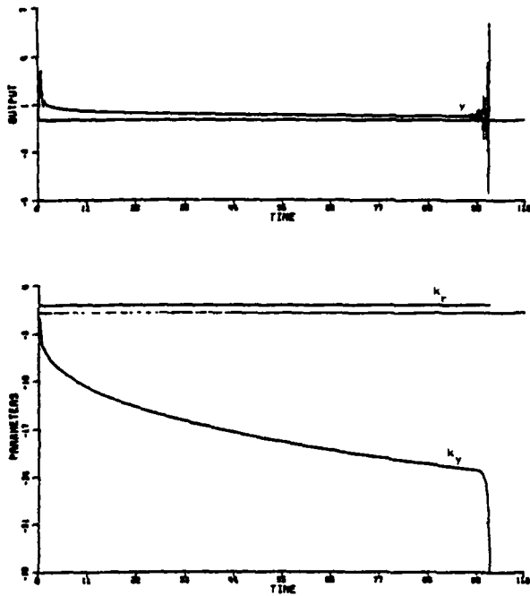
Figure 9: Simulation of CAL with unmodeled dynamics, r(t)=0.0 , and d(t)=3.0 \times 10^{-6} . (System eventually becomes unstable.)
