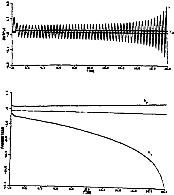
Figure 7: Simulation of CAL with unmodeled dynamics, r(t)=0.3 , and d(t)=5.59 \times 10^{-6} \sin 16.1t . (System eventually becomes unstable.)
