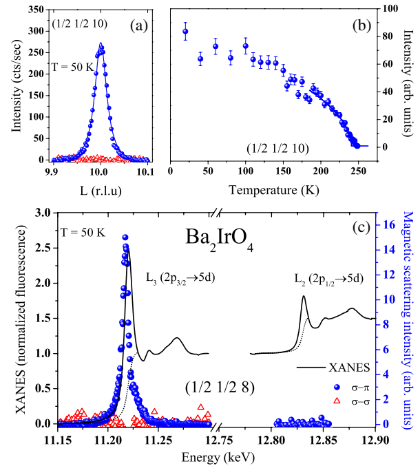
FIG. 2 (color online). (a) L scans across the (\frac{1}{2}\ \frac{1}{2}\ 10) magnetic reflection, T = 50\text{ K} in \text{Ba}_2\text{IrO}_4 . (b) The temperature dependence of the (\frac{1}{2}\ \frac{1}{2}\ 10) magnetic reflection in \text{Ba}_2\text{IrO}_4 . The solid blue line is a fit to a power law. (c) Resonant enhancement of the (\frac{1}{2}\ \frac{1}{2}\ 8) magnetic reflection across the L_{2,3} edges at T = 50\text{ K} in \text{Ba}_2\text{IrO}_4 . The solid black line shows the XANES spectra normalized to the number of initial states. The blue spheres and red triangles show the intensity of the (\frac{1}{2}\ \frac{1}{2}\ 8) reflection. The black dashed line demarcates the integrated white line used to calculate the branching ratio.
