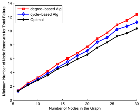
Fig. 4. Comparing different algorithms with optimal solution
