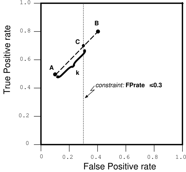
Figure 10: Interpolating classifiers
