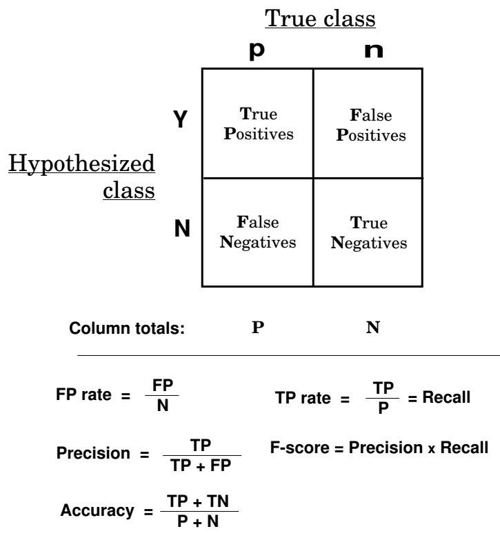
Figure 1: A confusion matrix and several common performance metrics that can be calculated from it
