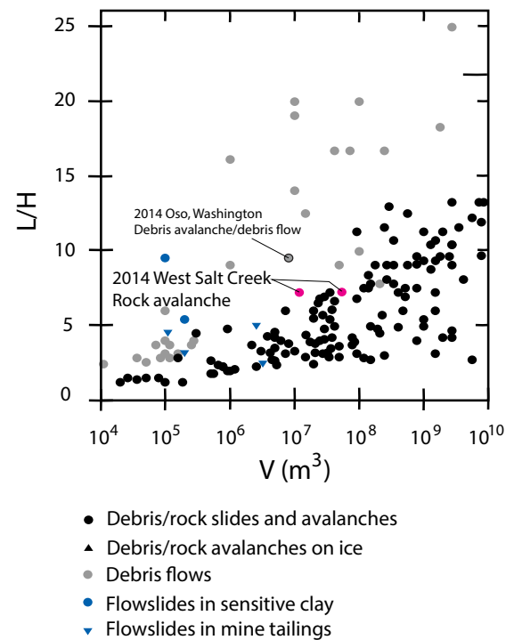
Figure 11. Comparison of mobility index values ( L is the maximum length traveled, H is the maximum elevation traveled, and V is landslide volume) for the West Salt Creek rock avalanche with those of other fast-moving landslides (modified from Iverson et al. [2015] using data from Carasco-Nunez et al. [1993], Corominas [1996], Iverson [1997], Dawson et al. [1998], Legros [2002], and Zanchetta et al. [2004]). Two dots for West Salt Creek represent the total combined volume of the slump block and mobilized rock avalanche ( 54.5 \pm 13.0 \text{ Mm}^3 ) and volume of the mobilized rock avalanche alone ( 11.5 \pm 0.1 \text{ Mm}^3 ). The recent Oso, Washington, debris avalanche is shown for reference. Sensitive clay is a type of clay that is prone to a sudden loss of strength when it is disturbed.
