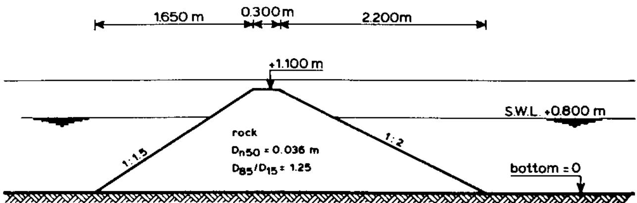
Figure 3.13 Tested homogeneous structure.
