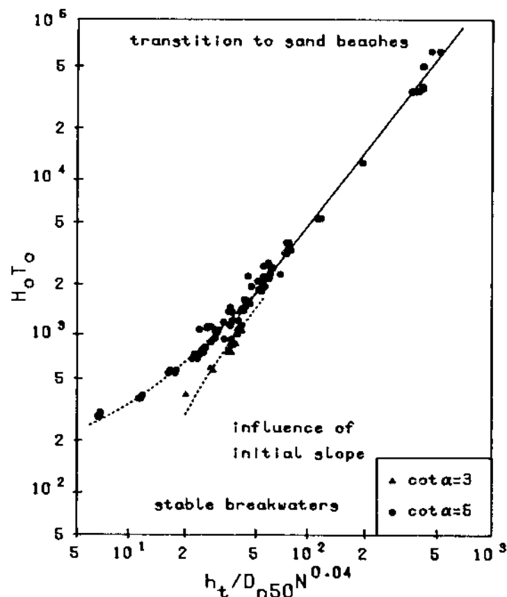
Figure 4.26 Relationship between transition height, h_t , and H_0T_0
