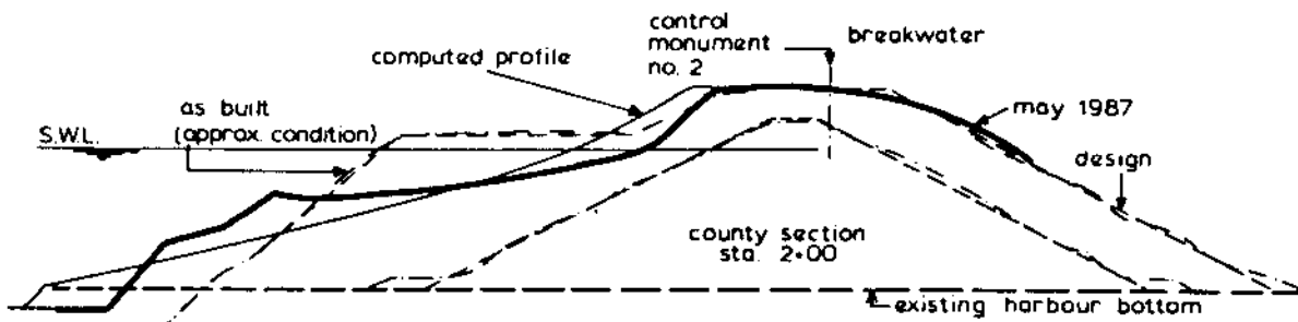
Figure 4.46 Verification on prototype berm breakwater measurements
