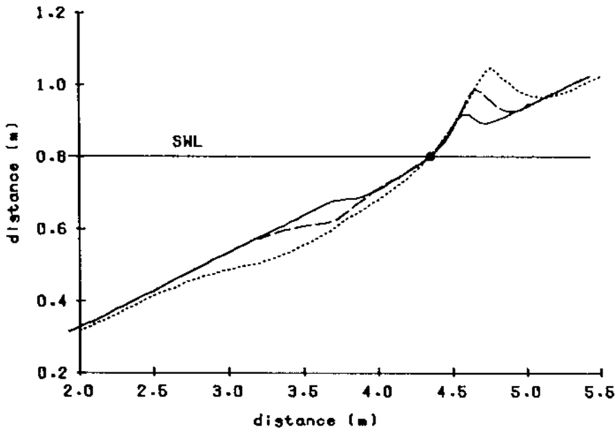
Figure 4.4 Influence of wave period
