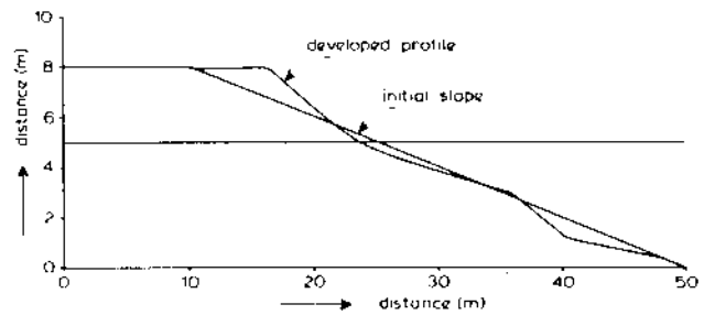
gravel beach H/\Delta D = 20 - 500
