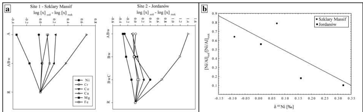
Fig. 5 Distribution of elements in soil horizons relative to the parent rocks (a) and the relationship between [\text{Ni}/\text{Al}]_{\text{soil}}/[\text{Ni}/\text{Al}]_{\text{rock}} and \delta^{60}\text{Ni} in soils (b)
