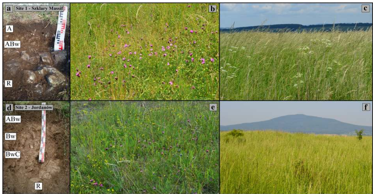
Fig. 2 Studied areas: (a-c) the Szklary Massif (site 1): (a) soil profile, (b) xerothermic grassland, (c) expansion of Calamagrostis epigejos and Arrhenatherum elatius ; (d-f) Jordanów (site 2): (d)
