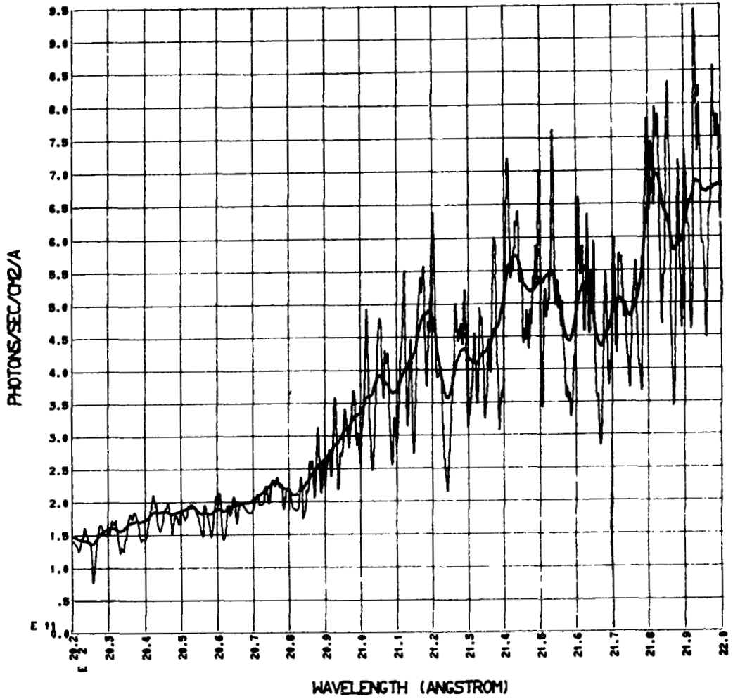
Figure E-1. High Resolution Solar Spectrum (Brinkmann et al. 1966) and Smoothed (4.6Å) Spectrum.
