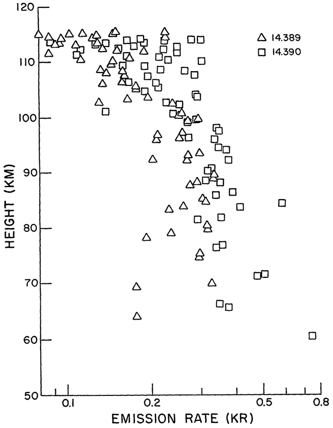
Figure IV-4. Emission rate of (2,0) Gamma Band for Both Flights. Ascent and Descent Leg Data Are Included, With No Distinction.
