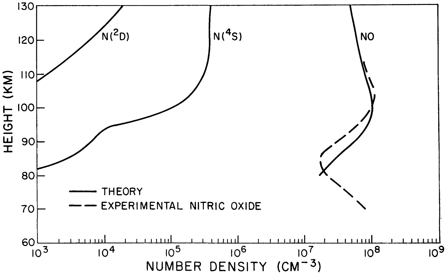
Figure V-1. Photochemical Equilibrium Density Profiles for NO , N(^4S) and N(^2D) . Experimental NO Profile from Flight 14.389.
