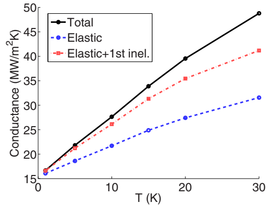
FIG. 3. (Color online) Interfacial conductance as a function of temperature for the mass-mismatched Lennard-Jones interface. The total conductance is G = Q/(A\Delta T) , where Q is the energy input (output) in the left (right) heat bath. The elastic conductance is \int_0^\infty g^{\text{el}}(\omega)d\omega/(2\pi) [Eq. (18)] and the first-order inelastic addition to the elastic conductance is \int_0^\infty g^{\text{inel}}(\omega)d\omega/(2\pi) [Eq. (19)]. Only elastic transmission processes contribute to the conductance at very low temperatures, but the importance of inelastic processes quickly increases with increasing temperature. The temperature change \Delta T at the interface has been calculated as described in the caption of Fig. 2.
