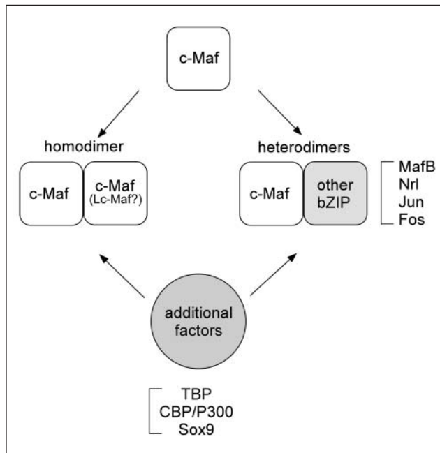
Figure 2. Different types of c-Maf binding interactions. c-Maf can form homodimers as well as heterodimers with other bZIP transcription factors. In addition, several factors, including general transcription factors (TBP), cofactors (CBP), and specific transcription factors (Sox9), interact with c-Maf.
