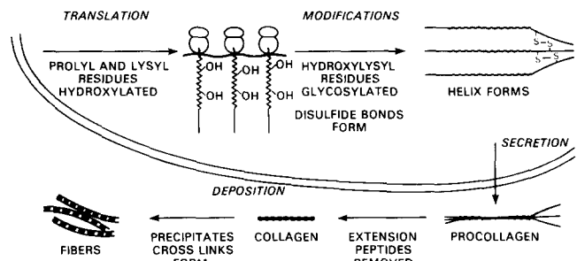
FIGURE 1 Synthesis and maturation of collagen. Certain prolyl and lysyl residues on the nascent chains are hydroxylated by specific enzymes. Although the hydroxylation begins on the nascent chains, it can continue after completion and release of the chains, until the triple helix forms. Helix formation also terminates glycosylation of hydroxylysyl residues. The procollagen molecule is then secreted from the cell where extracellular or membrane-bound enzymes remove the noncollagenous extension peptides. The collagen molecules are enzymatically cross-linked to form stable fibers.
