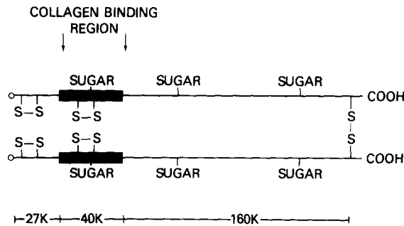
FIGURE 2 Schematic model of the fibronectin molecule including the location of specific domains. Peptides containing the collagen-binding site (40K), the transglutaminase cross-linking site (27K), and the cell-binding site (160K) are shown in their probable locations in the molecule (11, 57, 154, 210). Some or all of the sugars are in the 40,000-dalton region (154, 210). The position of the S-S bonds is from Wagner and Hynes (233).
