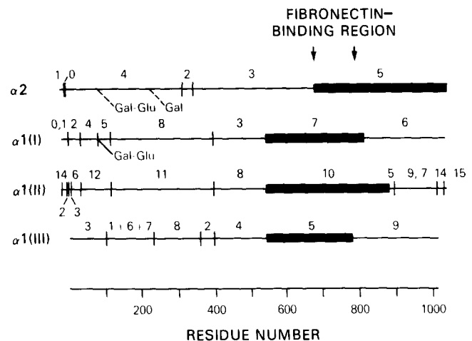
FIGURE 5 Activity of various cyanogen bromide-derived peptides of collagen \alpha -chains in binding fibronectin. The numbers between the vertical lines indicate the cyanogen bromide peptide number. The major peptides active in binding fibronectin are shaded (■). Data on \alpha 2(I) , \alpha 1(I) , \alpha 1(II) are from Dessau et al. (37). Data on \alpha 1(I) and \alpha 1(II) are from Kleinman et al. (119). Data on \alpha 1(III) are from Kleinman and McGoodwin (unpublished observations).
