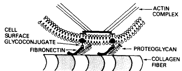
FIGURE 6 Schematic model of an adhesion site. Collagen fibers contain specific sites to which the fibronectin molecule binds. The fibronectin molecule contains a region that recognizes collagen and another region that recognizes the cell surface. The cell surface receptor is thought to be a glycoconjugate, possibly a glycolipid that interacts with cytoskeletal elements in some as yet unknown manner. Proteoglycans are also present and stabilize the interaction. The components of this model are not necessarily to scale.
