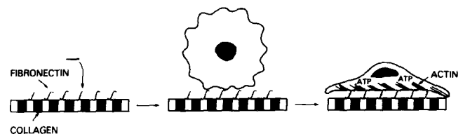
FIGURE 3 Schematic model of fibronectin-mediated cell adhesion to collagen in vitro . Fibronectin first binds to a specific sequence of amino acids on the collagen chain (113, 120, 165). Then the cells in the presence of \text{Ca}^{++} or \text{Mg}^{++} bind to the fibronectin-collagen complex (115) and spread.
