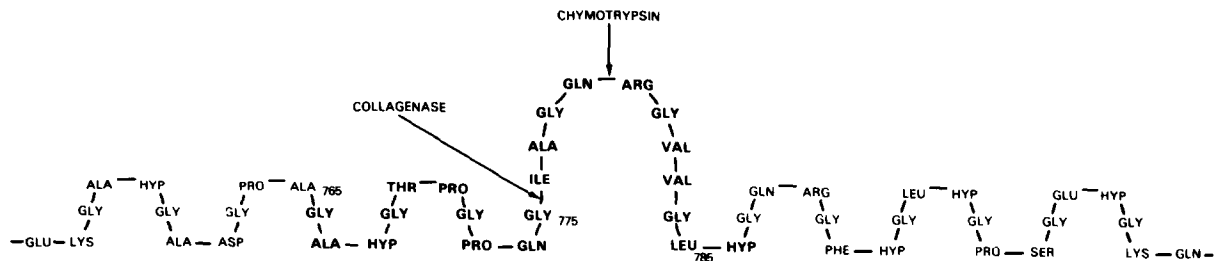
FIGURE 4 Amino acid sequence of the collagen \alpha 1(I) -chain known to bind fibronectin. The secondary structure of the active region (residues 774–785) is diagrammatically depicted as being more open than the remainder of the molecule whose tight helical coil is depicted with regular curves. The fibronectin-binding site (residues 766–786) is shown in heavy letters.
