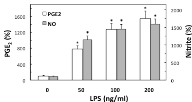
Figure 1. Effect of H. pylori LPS on PGE 2 and nitrite production in rat gastric mucosal cells. The cells were treated with the indicated concentrations of the LPS and incubated for 16 h. Values represent the means \pm SD of five experiments. * P < 0.05 compared with that of control (LPS - 0).
