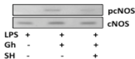
Figure 7. Effect of ghrelin (Gh) and Akt kinase inhibitor, SH-5 (SH), on H. pylori LPS-induced changes in cNOS phosphorylation in gastric mucosal cells. The cells were treated with ghrelin at 0.5 \mu\text{g/ml} , or Akt inhibitor, SH-5 (30 \mu\text{M} ) + Gh, and incubated for 16 h in the presence of 100 ng/ml LPS. Cell lysates were resolved on SDS-PAGE, transferred to nitrocellulose, and probed with phosphorylation-specific cNOS (pcNOS) antibody, and after stripping reprobated with anti-cNOS antibody. The immunoblots shown are representative of three experiments.
