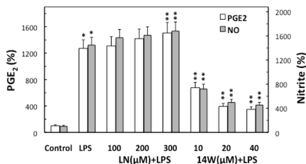
Figure 3. Effect of nitric oxide synthase inhibitors on H. pylori LPS-induced changes in the production of PGE 2 and nitrite by gastric mucosal cells. The cells, preincubated with the indicated concentrations of cNOS inhibitor, L-NAME (LN), or iNOS inhibitor, 1400 W, were treated with the LPS at 100 ng/ml and incubated for 16 h. Values represent the means \pm SD of five experiments. * P < 0.05 compared with that of control. ** P < 0.05 compared with that of LPS alone.
