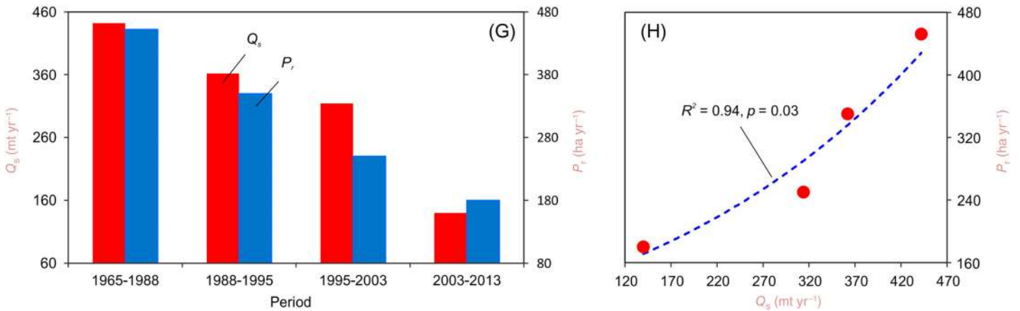
Fig. 5. Reduction in the progradation rate of the marshes in Eastern Chongming (EC) in response to the decline in the sediment discharge of the Yangtze River. (A-F) Marsh-mudflat boundaries in different years. (G) Time-averaged sediment discharge ( Q_s ) of the Yangtze River and progradation rate ( P_r ) of salt marshes in Eastern Chongming. (H) The correlation between P_r and Q_s in subplot (G).
