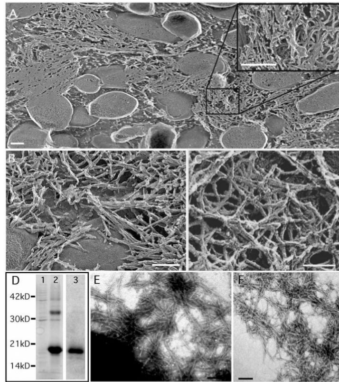
Fig. 1. High-resolution deep-etch EM micrographs of curliated E. coli and purification of curli fibers. (A and B) Representative freeze-fractured micrographs that have been rotary shadowed with platinum. The inset in (A) shows curli fibers. (C) MC4110 was absorbed onto glass and deep-etched without being fractured before rotary shadowing with platinum. (D) Coomassie stain SDS-PAGE of curli samples isolated from E. coli strain MC4100. Lanes 1 and 2 contain 40 \mu g of S6 wild-type curli without and with FA treatment, respectively. Lane 3 contains 20 \mu g of FA-treated GP curli. Molecular size markers (in kilodaltons) are indicated on the left. (E) Negative-stain EM micrographs of MC4100 grown on YESCA plates at 26°C for 48 hours. (F) Negative-stain EM micrograph of purified wild-type S6 curli. Bars: (A), 400 nm; (B) and (C), 60 nm; (E) and (F), 200 nm.
