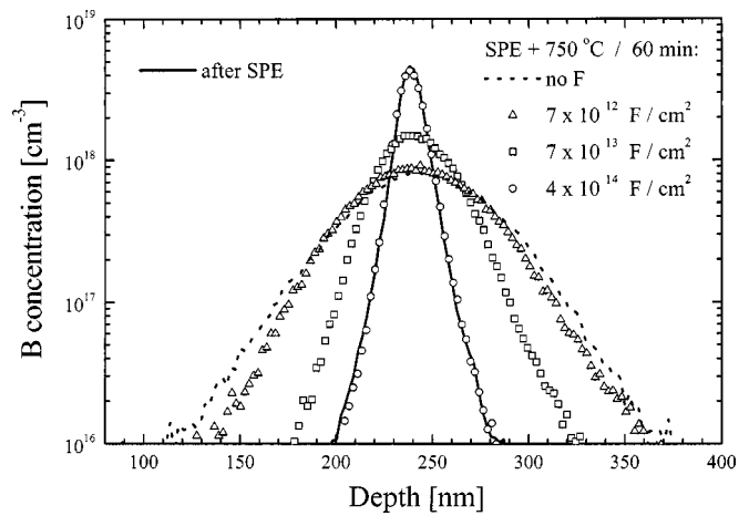
FIG. 2. B diffused profiles for the three different doses of F implantation after SPE plus thermal anneals (open symbols) at 750 °C/60 min. B profile for a similar sample without F is also shown for reference (dashed line).
