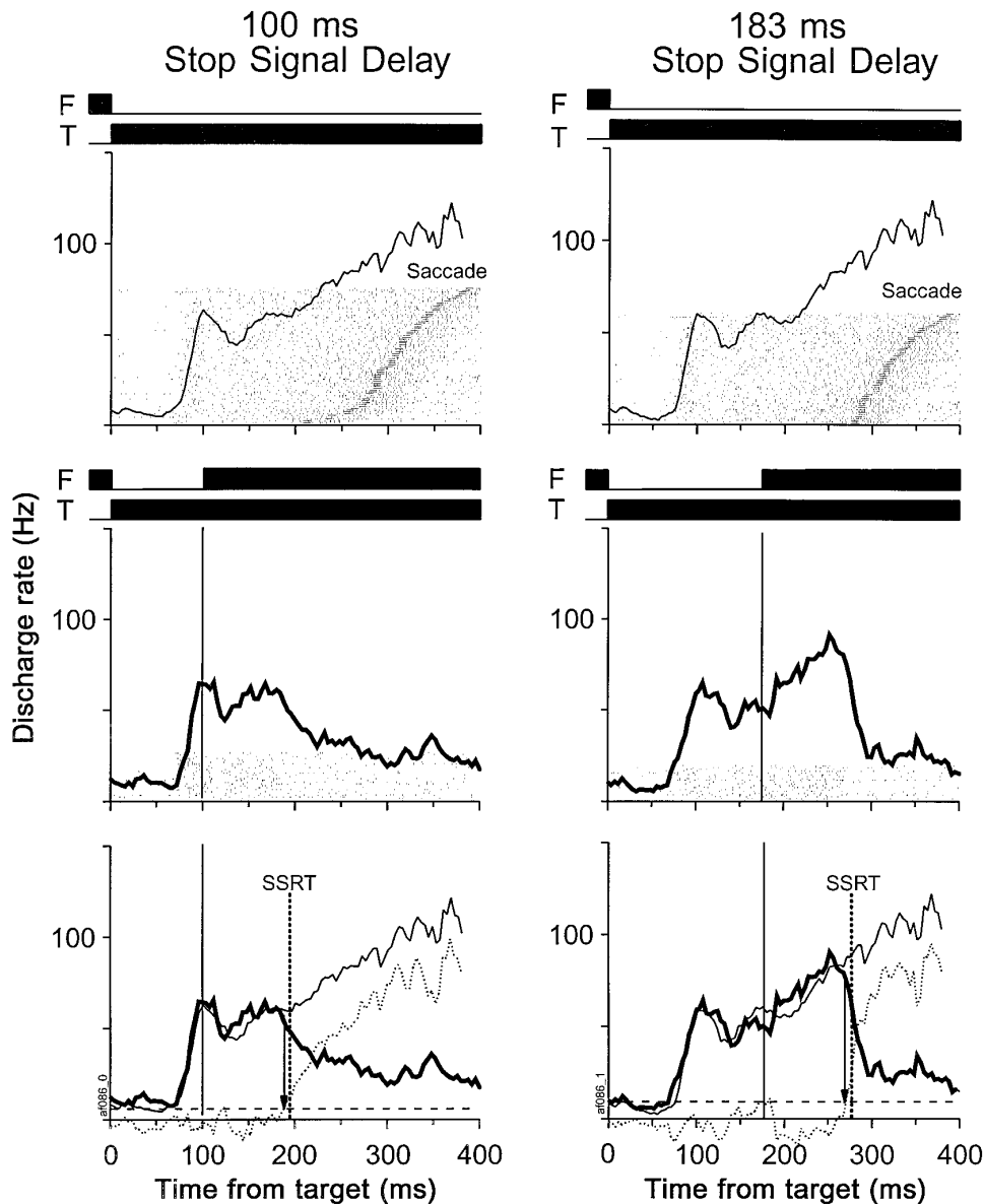
FIG. 5. Activity of a representative cell with movement-related activity aligned on the time of target presentation. Trials collected during the countermanding task with stop-signal delays of 100 ms ( left ) and 183 ms ( right ) are shown. No-stop-signal trials that are latency matched to cancelled trials are shown ( top 2 panels ). Cancelled trials also are shown ( middle 2 panels ). Conventions as in Fig. 4, except the horizontal tickmarks in the top panels indicate the time of saccade initiation. Spike density functions for cancelled (—) and latency-matched no-stop-signal trials (—) are shown. Bottom 2 panels : comparison of the spike density functions during cancelled and latency-matched no-stop-signal trials. ···, differential spike density function. |, time of presentation of the stop-signal; †, estimated SSRT; — —, discharge rate 2 SD above the mean of the differential spike density function rate in the interval of fixation 600 ms before the presentation of the target; ‡, time at which the differential activity became significant.
