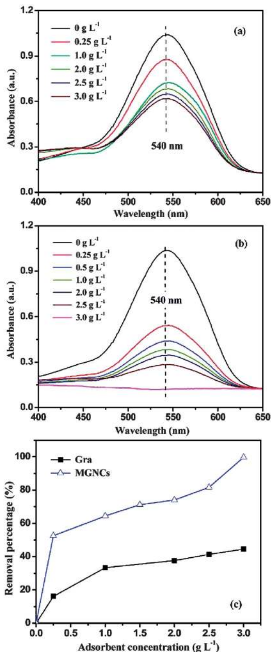
Fig. 10 UV-Vis absorption of the solutions after treated with (a) different loadings of graphene (Gra), (b) different loadings of MGNCs, and (c) \text{Cr(VI)} removal percentage based on different loadings of Gra and MGNCs. [\text{Cr(VI)}] = 1000 \mu\text{g L}^{-1} , pH 7, treatment time: 5 min. Reproduced with permission from ref. 242, copyright (2011) American Chemical Society.
