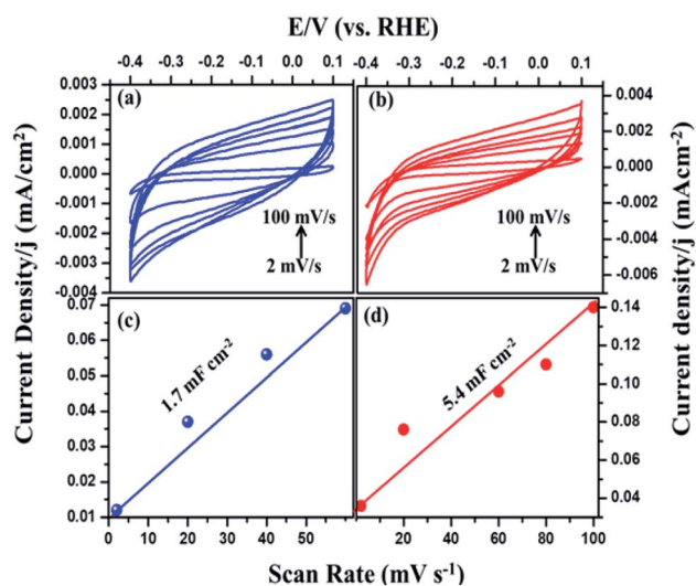
Fig. 9 Cyclic voltammety of MIL-53(Fe) (a) dehydrated and (b) hydrated and (c and d) plots showing the extraction of the C_{dl} for MIL-53(Fe)/dehydrated and hydrated.
