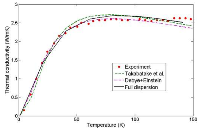
FIG. 5. Lattice thermal conductivity of \text{LaFe}_4\text{Sb}_{12} plotted versus temperature. Experimental data are taken from Takabatake et al. 31 Three models based on relaxation times approximation are used to fit the experimental data. The first two models are Debye + Einstein models which are using Debye dispersion and adding a resonance scattering term for Einstein frequencies. These two models are using different expressions for resonance scattering (Eq. (7) is used by Takabatake et al. and Eq. (8) is used for the plot labeled as Debye + Einstein). The third model is based on full dispersion. All fitting parameters for this plot are listed in Table I.
