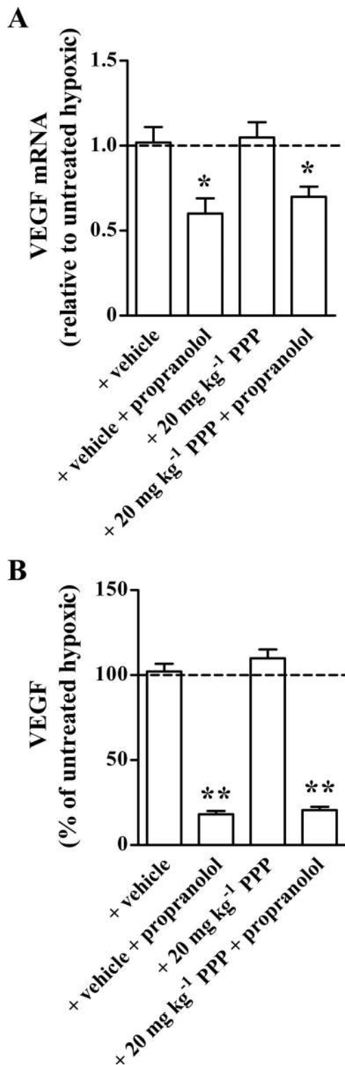
FIGURE 10. VEGF expression in OIR mice treated with picropodophyllin (PPP), an inhibitor of IGF-1R phosphorylation. (A) QPCR evaluation of VEGF mRNA and (B) ELISA quantitation of VEGF content in the hypoxic retina after treatment with vehicle or PPP (20 mg kg -1 ) either alone or in combination with propranolol at 20 mg kg -1 . Vehicle or PPP did not influence hypoxic levels of VEGF mRNA and protein. VEGF mRNA and protein levels after PPP+propranolol were not significantly different from those measured after vehicle+propranolol. In QPCR experiments, data were analyzed by the C t method with Rp113a used as the internal standard. Each histogram
