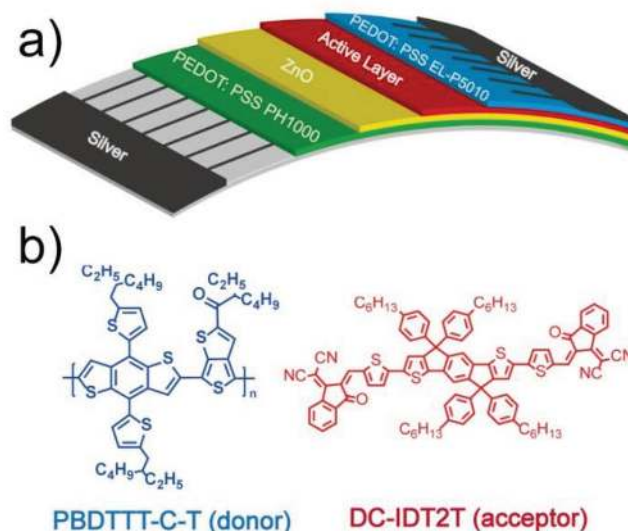
Figure 1. a) Structure of roll-coated solar cells, and b) molecular structures of PBDDTT-C-T (donor) and DC-IDT2T (acceptor).
