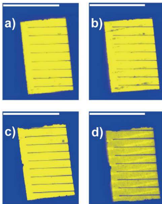
Figure 7. LBIC images of a,b) PBDTTT-C-T/DC-IDT2T and c,d) PBDTTT-C-T/PC 71 BM films a,c) before and b,d) after exposing to sunlight for 180 h. All the scale bars are 1 cm.
