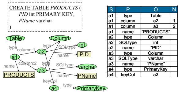
Figure 3: Sample model shown as graph and 4-tuples
