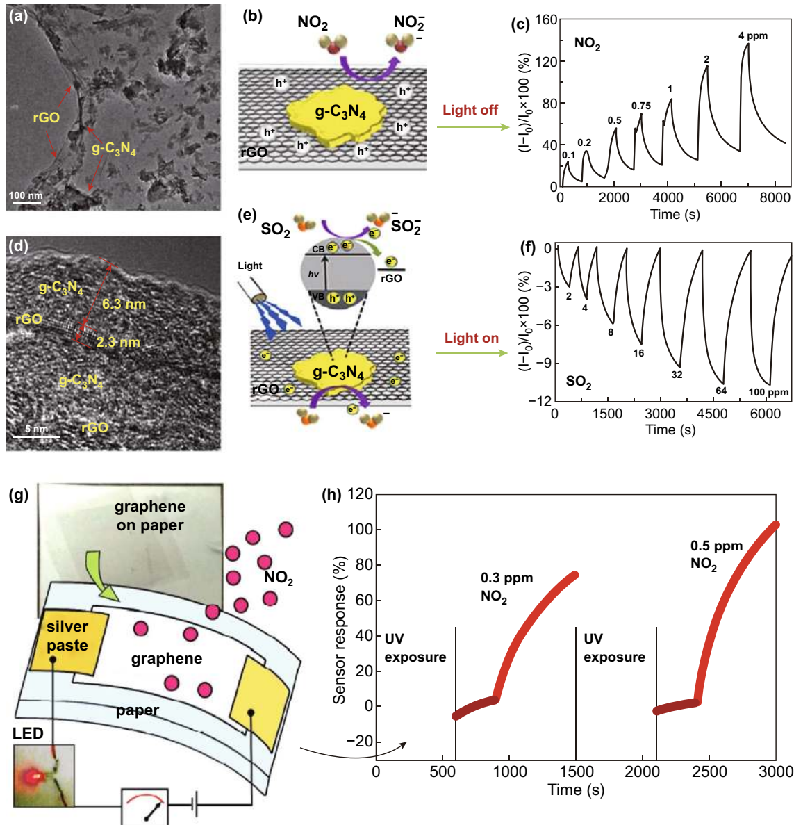
Fig. 11 SEM image of g-C 3 N 4 /rGO hybrid a in low, and d high magnification. b Schematic representation of charge transfer between g-C 3 N 4 /rGO hybrid and NO 2 under dark condition. c Transient gas response of the hybrid sensor to NO 2 gas under dark condition. e Schematic representation of charge transfer between g-C 3 N 4 /rGO hybrid and SO 2 under UV light illumination. f Transient gas response of the hybrid sensor to SO 2 gas under UV light illumination. Reproduced with permission [103]. Copyright 2017, American Chemical Society. g Schematic illustration of a graphene sensor on paper substrate. h Gas response of the flexible graphene sensor. Reproduced with permission [104]. Copyright 2015, American Chemical Society
