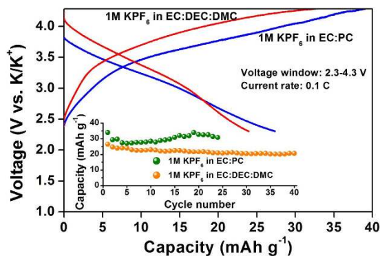
Figure 4. K-intercalation studies of \text{rGO}/\text{K}_2[(\text{VO})_2(\text{HPO}_4)_2(\text{C}_2\text{O}_4)] composites. Galvanostatic charge discharge cycling showing voltage vs. capacity profiles for fifth cycle using different electrolytes in the voltage range, 2.3–4.3 V vs. \text{K}/\text{K}^+ at a current density of 11 \text{ mA g}^{-1} ( \sim 0.1 \text{ C} ). The inset figure shows the variation of capacity with cycle number.
