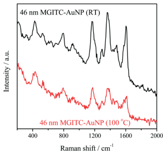
Fig. 6 SERS spectra of MGITC (20 nM) adsorbed on room temperature and 100 °C seed mediated AuNPs under 633 nm excitation. MGITC-AuNPs were prepared by quickly adding \approx 1.5 \mu L of 14 \mu M MGITC solution to 1 mL AuNP suspension ( 5.4 \times 10^{10} particle per mL).
