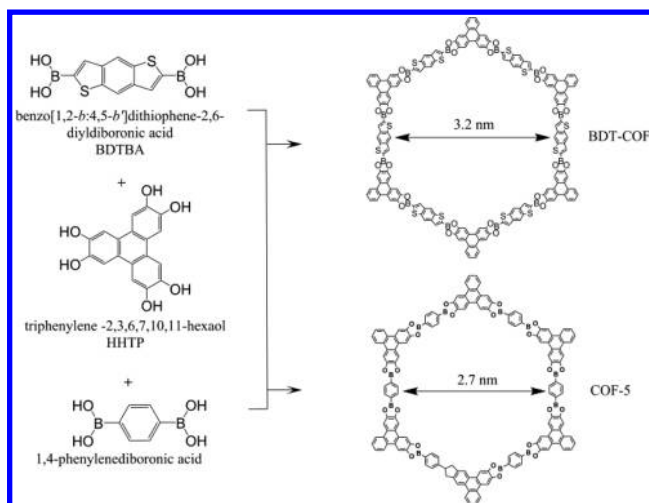
Figure 1. Schematic representation of BDT-COF and COF-5.
