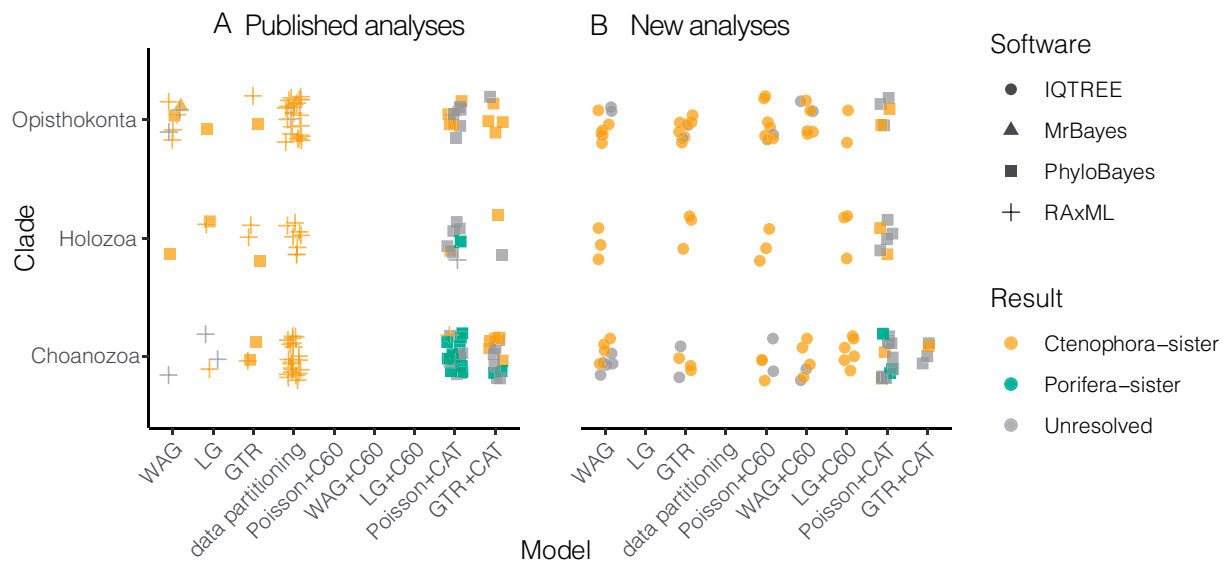
FIG. 3. Summary of phylogenomic results from previous studies and reanalysis conducted in this study. Each point represents a phylogenetic analysis with a support of bootstrap values less than 90% or a posterior probability less than 95% are considered as unresolved. The clades are organized with increased outgroup sampling higher on the vertical axis, and the models are organized in general by increasing complexity in terms of numbers of parameters to the right on the horizontal axis. (A) Analyses transcribed from the literature (related to supplementary table S1, Supplementary Material online). (B) New phylogenomic analyses conducted in this study (related to supplementary table S2, Supplementary Material online). Over 1,011,765 CPU hours (~115 CPU years) were used for this study.
