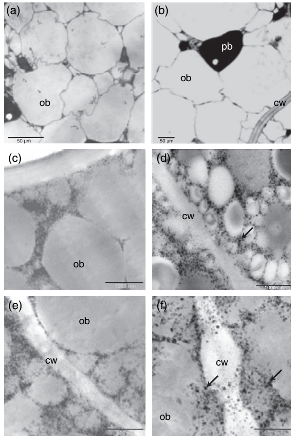
Figure 3. Subcellular localization of \text{H}_2\text{O}_2 in sunflower embryonic axes. (a, b) Dormant and non-dormant axes, respectively, viewed by TEM without \text{H}_2\text{O}_2 staining (sections not infiltrated by \text{CeCl}_3 ). (c, e) and (d, f) Dormant and non-dormant axes, respectively, viewed by TEM with \text{CeCl}_3 -staining. \text{H}_2\text{O}_2 is visualized as black spots corresponding to electron-dense cerium perhydroxide precipitates (arrows). Abbreviations: cw, cell wall; ob, oil body; pb, protein body. Scale bars represent 50 \mu\text{m} (a,b), 1000 nm (c,d) and 500 nm (e,f).
