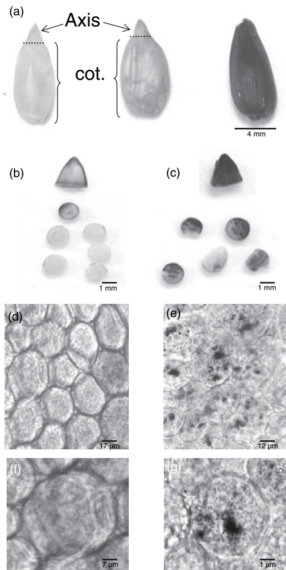
Figure 2. Localization of O_2^{\cdot -} in sunflower embryonic axes.
