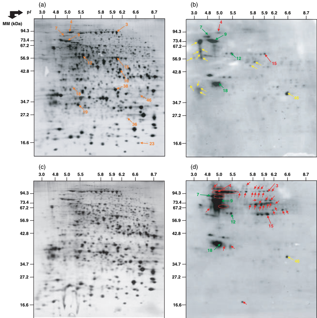
Figure 5. Two-dimensional profiles of protein abundance and oxidation in axes of dry dormant and non-dormant sunflower seeds.
