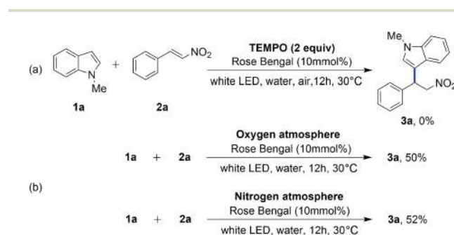
Scheme 3 Control experiment.
