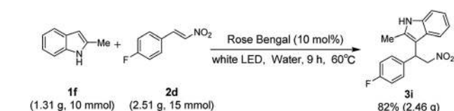
Scheme 2 Gram scale Friedel–Crafts alkylation reaction.
