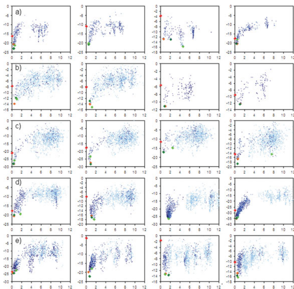
Fig. 2. Results of cross-docking benchmark of pairs of complexes A/B: (a) 1aq1/1dm2, (b) 1dbj/2dbl, (c) 1dwc/1dwd, (d) 1fm9/2prg, (e) 1p8d/1pq6, (f) 1p8d/1pq6, (g) 1ppc/1pph, (h) 1pq6/1pqc, (i) 2ctc/7cpa, (j) 4tim/6tim: The diagrams show from the left to the right ligand A docked in protein A, ligand A docked in protein B, ligand B docked in protein A, and ligand B docked in protein B. The ROSETTALIGAND binding energy is shown on the y -axis and the RMSD in Ångströms on the x -axis. In all diagrams the energy of the crystal structure (red diamond), the minimized native structure (orange diamond), the lowest energy model obtained utilizing the crystal structure conformation of the ligand (dark green diamond), and the lowest energy model obtained including ligand flexibility (light green diamond) are shown. All other models obtained from the crystal structure conformation of the ligand are shown as dark blue points and models obtained including ligand flexibility are marked with light blue points.
