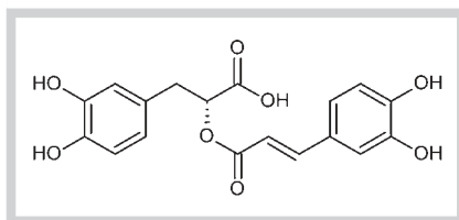
Fig. 1 (R)-(+)-rosmarinic acid.
