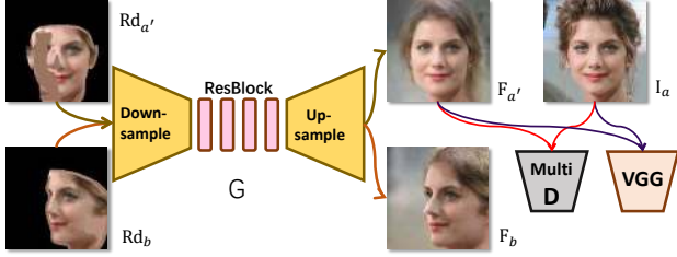
Figure 5: Our render-to-image module. Rendered images Rd_{a'} and Rd_b are sent into the generator G to get the results F_{a'} and F_b . Losses are conducted between generated F_{a'} and the ground truth I_a through the discriminator and the pretrained VGG network.
