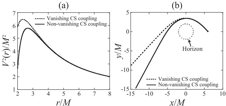
Fig. 1. (a) Potential V^2(r) . (b) Particle trajectories in the equatorial plane. The starting point is indicated by a small filled circle. The results in the presence of the CS coupling are denoted by solid curves, while the results in the absence of the CS coupling are denoted by dashed curves. In both figures, we assume E = 2.35 , L/M = 10.0 , J/M^2 = 0.5 , and \tilde{\ell}^2 = 0.1 .
