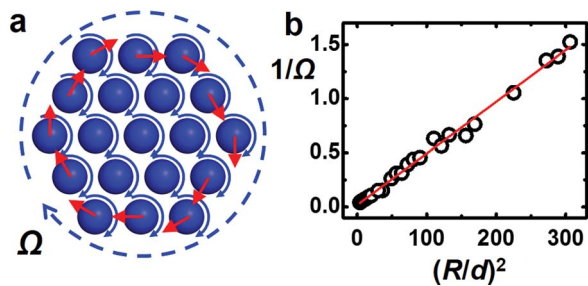
Fig. 3 Crystal rotation. (a) Schematic representation of the rotation mechanism. Particles at the edge experience an unbalanced hydrodynamic shear force tangent to the edge (circle of red arrows). (b) Inverse angular velocity 1/\Omega plotted as a function of (R/d)^2 , where R is the size of the crystal piece and d = 1.6 \mu\text{m} is the particle diameter in order to access the large crystal size. Red line is a linear fit.
