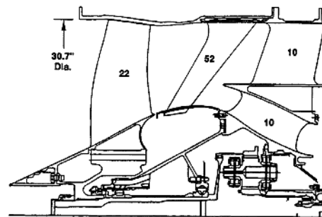
Figure 13.—TFE731 flow-path.
