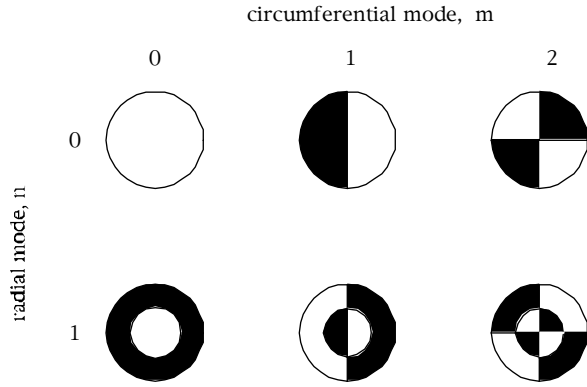
Figure 1.—Duct mode graphical representation.
