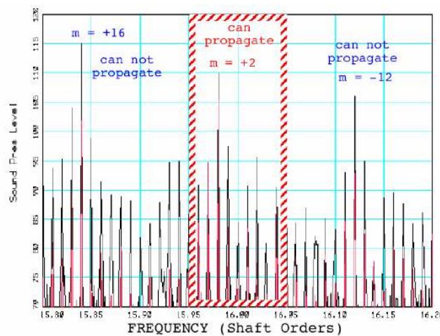
Figure 7.—Reduction of wake contamination due to installation of exhaust rake shields.
