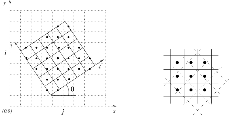
Fig. 1. Each text cell is matched against the pattern cell that covers the center of the text cell. As a consequence, some pattern cells may have to match several text cells simultaneously, whereas some others may not have to match any text cell at all (right).
