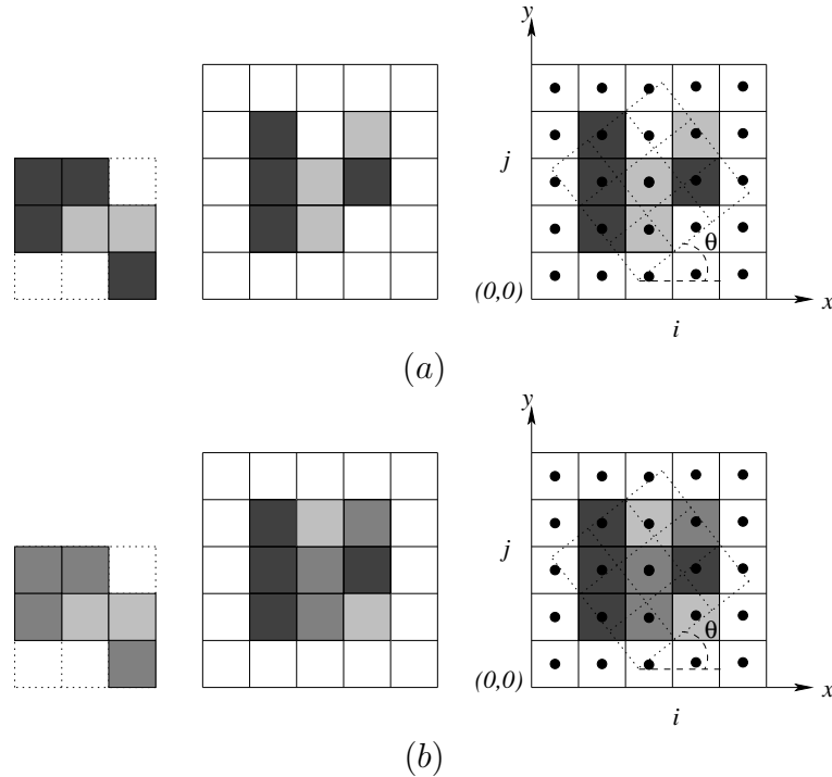
Fig. 2. Some examples of matches. In (a) we show a 3 \times 3 pattern over three gray levels, a 5 \times 5 text, and a rotated occurrence. Note that every text center covered by some pattern cell matches the color of the corresponding pattern cell, with the exception of the text cell in the third column and second row (counting from below). This text cell is light gray and is aligned with a white pattern cell. This alignment will be declared as an occurrence, for example, if we permit Hamming distance 1, as d_H(i, j, \theta, 0) = 1 . In (b) we illustrate matching with lighting invariance using four gray levels. The matching cells are the same as in (a) provided we shift all the gray levels of the text cells by t = 1 (assuming colors go from black = 0 to white = 3). That is, d_H(i, j, \theta, 1) = d_H^t(i, j, \theta) = 1 .
