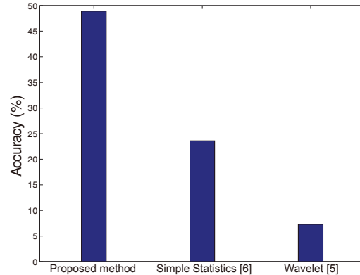
Fig. 4. The performance results of the proposed method compared to the other methods [5, 6]. The proposed method uses the setting of ‘combination’ (see Fig. 3).
