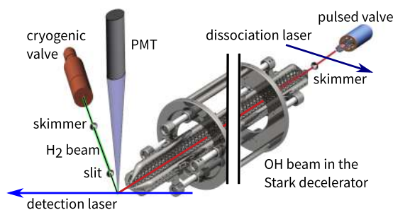
FIG. 1. This schematic drawing of the experimental apparatus shows the production and manipulation of the OH (red line) and H 2 (green line) packets before they enter the collision zone, which is depicted in the lower left part, where the OH packet out of the Stark decelerator cross the H 2 packet from the Even-Lavie valve, which is mounted on top of a helium cryostat. Scattered products were probed with the laser beam intersecting the collision zone (lower blue arrow).
