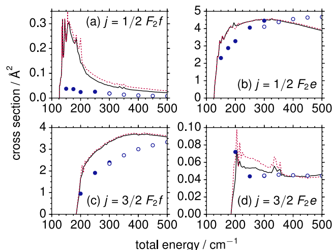
FIG. 3. State-to-state integral cross sections as a function of total energy for OH ( j_1 = 3/2 F_1 f to several low-lying F_2 levels) in collisions with para - \text{H}_2 ( j_2 = 0 \rightarrow 0 ). The solid and the dashed lines represent cross sections computed using the CCSD(T) and the MRCI PES's, respectively. The cross sections from calculations by Offer et al. (taken from Ref. 19) are plotted in dots (close-coupling calculations) or circles (coupled-states calculations).
