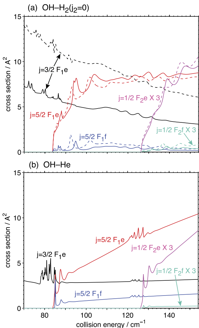
FIG. 13. Integral inelastic state-to-state cross sections for collisions of OH( X 2 Π, j 1 = 3/2 F 1 f ) with (a) H 2 ( j 2 = 0) and (b) He vs. collision energy over the range 75–150 cm -1 . The solid and dashed curves in panel (a) denote OH–H 2 calculations that included j 2 = 0 only and j 2 = 0 and 2, respectively, in the H 2 rotational basis. The cross sections were computed with PES's reported in Refs. 24 and 26, respectively.
