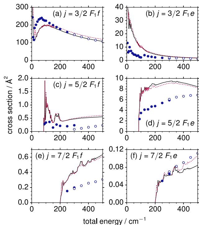
FIG. 2. State-to-state integral cross sections as a function of total energy for OH ( j_1 = 3/2 F_1 f to several low-lying F_1 levels) in collisions with para - \text{H}_2 ( j_2 = 0 \rightarrow 0 ). The solid and the dashed lines represent cross sections computed using the CCSD(T) and the MRCI PES's, respectively. The cross sections from calculations by Offer et al. (taken from Ref. 19) are plotted in dots (close-coupling calculations) or circles (coupled-states calculations).
