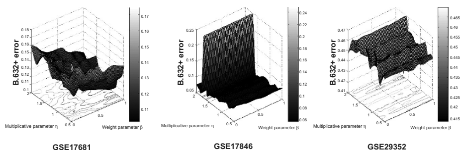
Figure 2 Variation of B.632+ error rate of the SVM with respect to multiplicative parameter \eta and weight parameter \beta .
