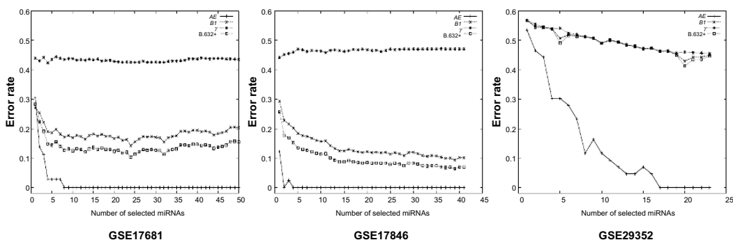
Figure 3 Error rate of the SVM obtained using the RSMRMS algorithm averaged over 50 random splits. Abbreviations: SVM, support vector machine; RSMRMS, rough set–based maximum relevance maximum significance; miRNA, microRNA; AE, apparent error; BI, bootstrap error; \gamma , no-information error; B.632+, B.632+ error.
