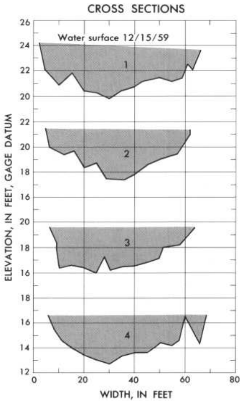
Plan sketch and cross sections, North Fork Cedar River near Lester, Wash.
