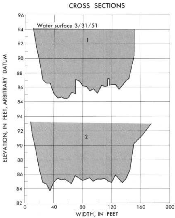
Plan sketch and cross sections, East Branch Ausable River at Au Sable Forks, N.Y.
