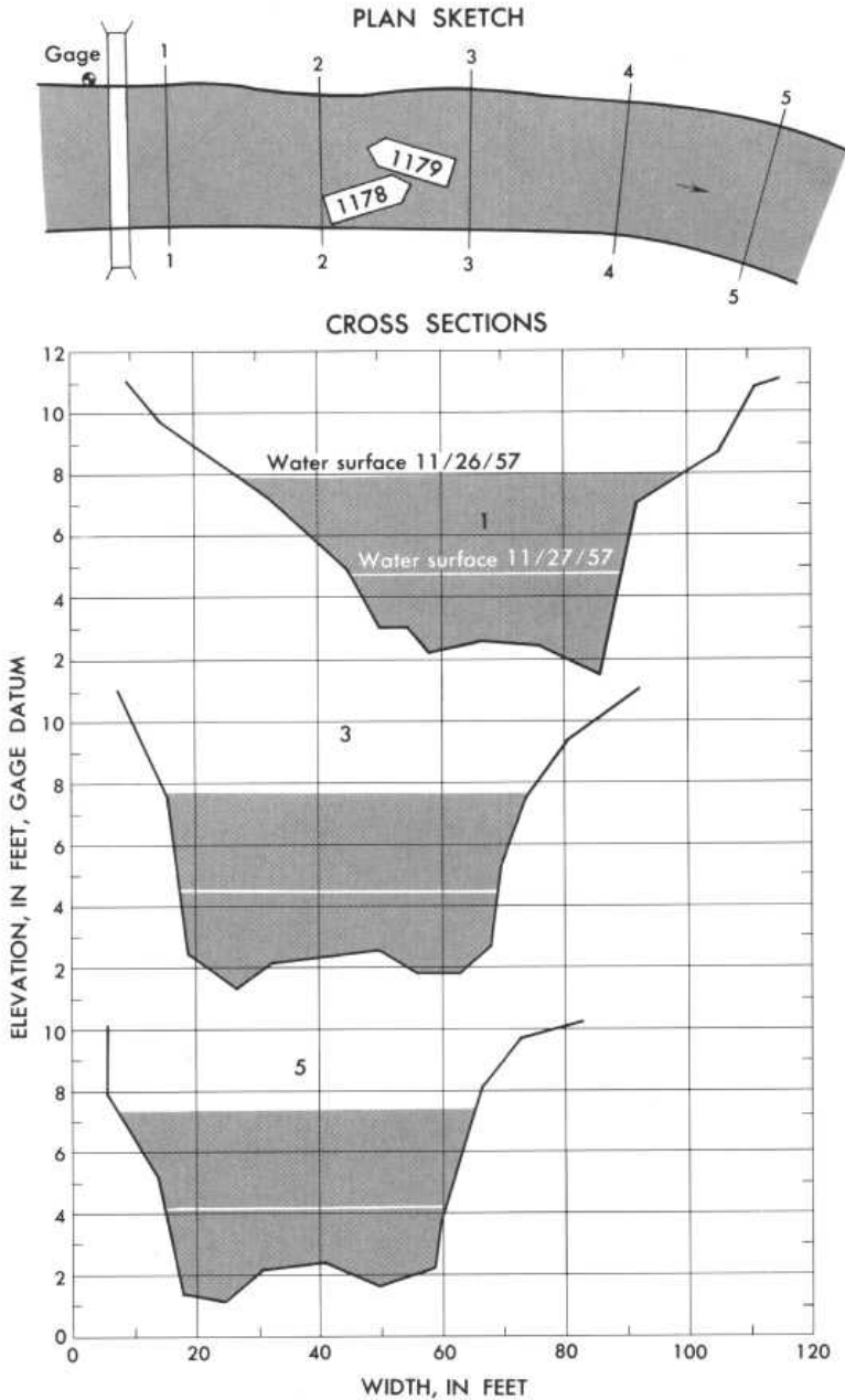
Plan sketch and cross sections, South Beaverdam Creek near Dewy Rose, Ga.
