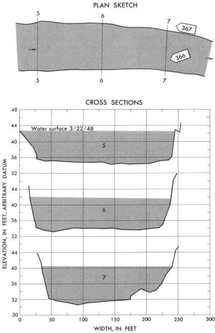
Plan sketch and cross sections, Beaver Kill at Cooks Falls, N.Y.
