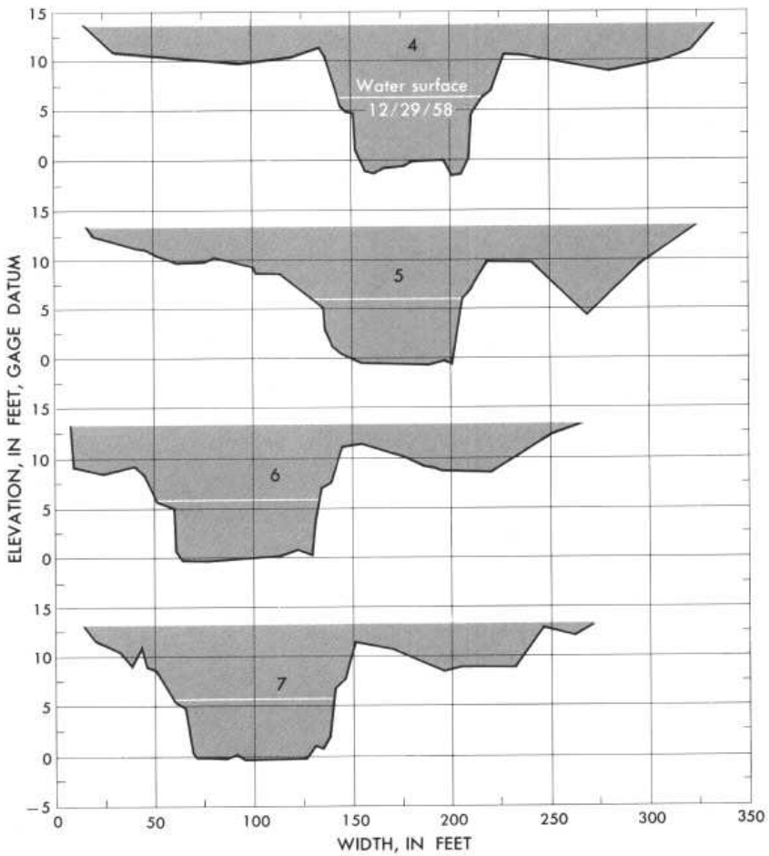
Plan sketch and cross sections, Haw River near Benaja, N.C.
