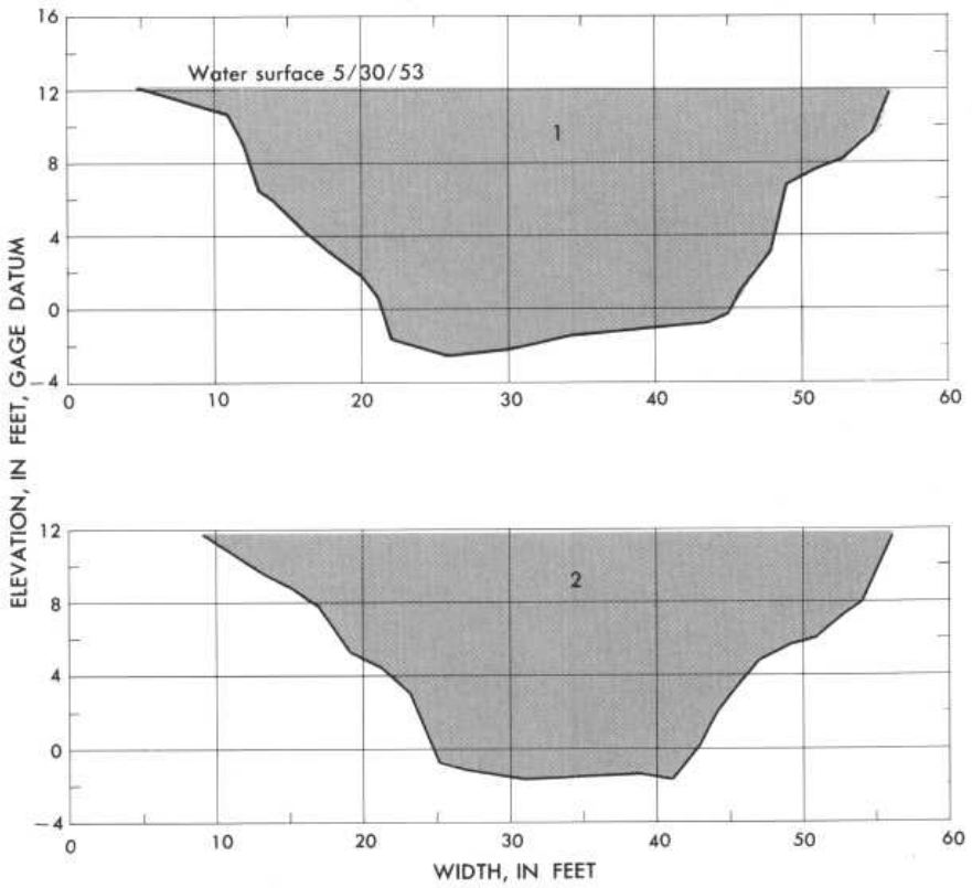
Plan sketch and cross sections, Beaver Creek near Newcastle, Wyo.
