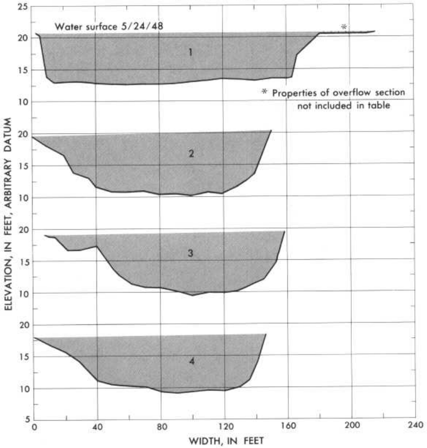
Plan sketch and cross sections, Moyie River at Eastport, Idaho.
