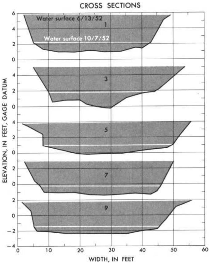
Plan sketch and cross sections, Provo River near Hailstone, Utah.
