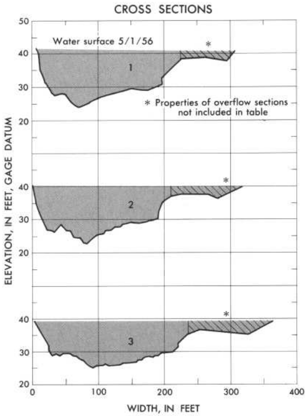
Plan sketch and cross sections, Yakima River at Umtanum, Wash.
