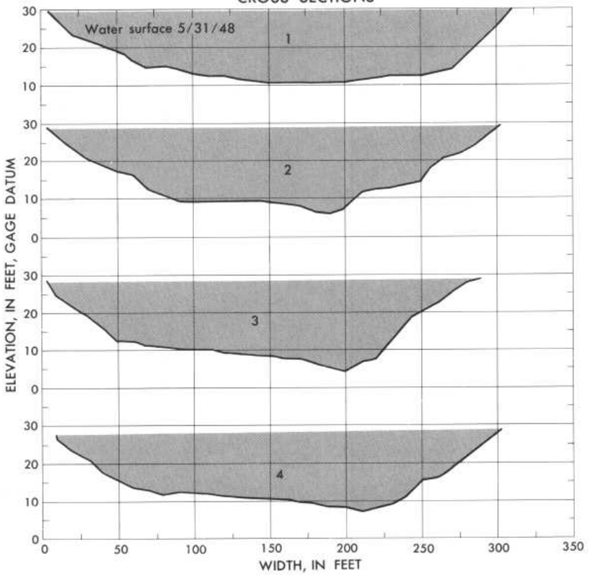
Plan sketch and cross sections, Spokane River at Spokane, Wash.
