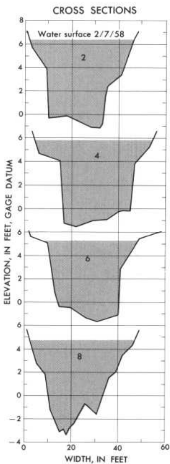
Plan sketch and cross sections, Murder Creek near Monticello, Ga.
