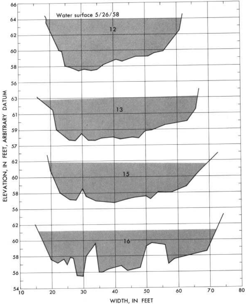
Plan sketch and cross sections, Clear Creek near Golden, Colo.
