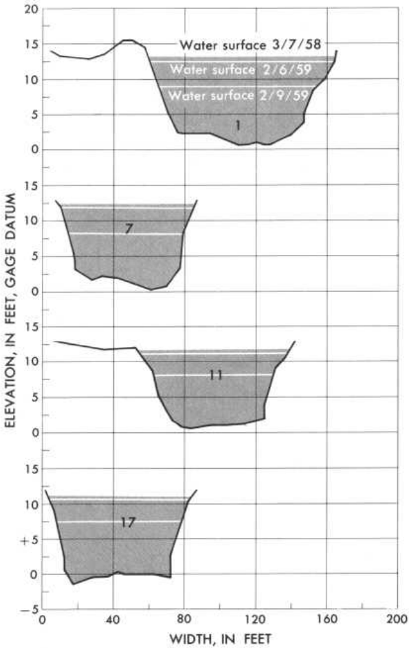
Plan sketch and cross sections, Tobesofkee Creek near Macon, Ga.
