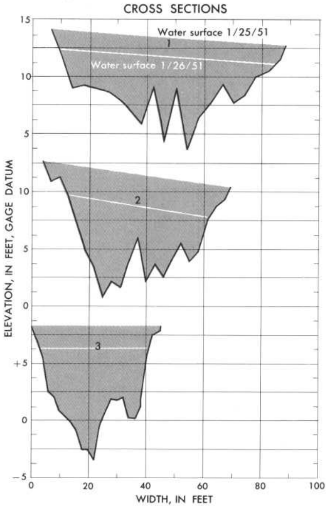
Plan sketch and cross sections, Cache Creek near Lower Lake, Calif.
