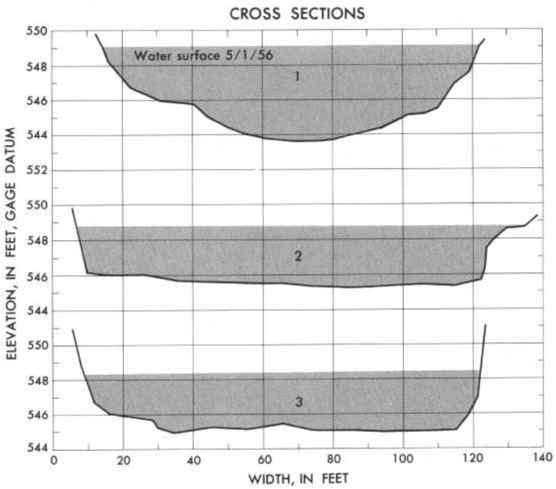
Plan sketch and cross sections, Middle Fork Vermilion River near Danville, Ill.
