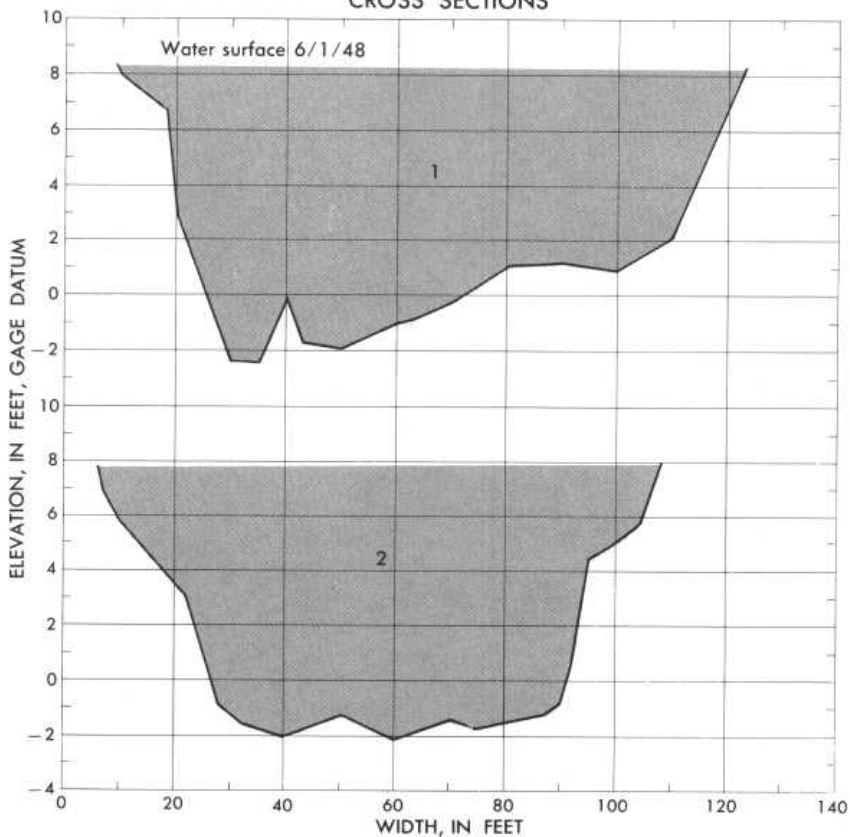
Plan sketch and cross sections, Bull Creek near Ira, Tex.
