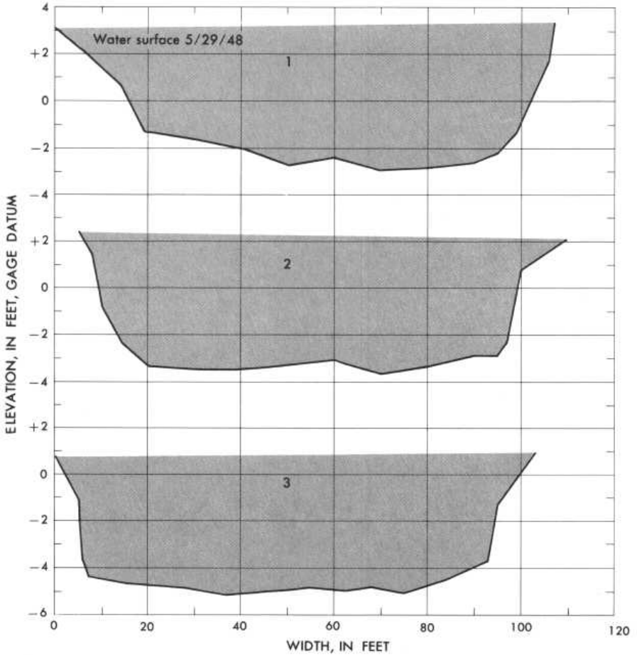
Plan sketch and cross sections, West Fork Bitterroot River near Conner, Mont.
