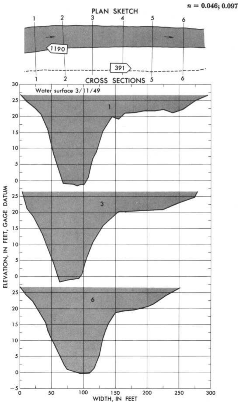
Plan sketch and cross sections, Rolling Fork near Boston, Ky. Dashed line shows limit of overbank flooding.
