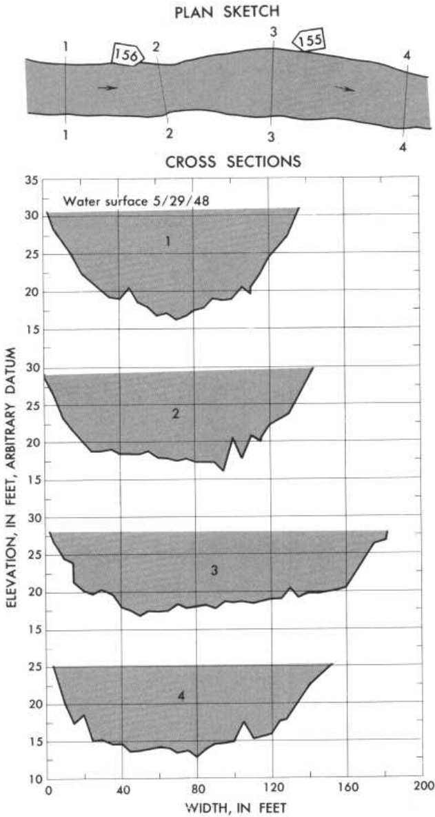
Plan sketch and cross sections, South Fork Clearwater River near Grangeville, Idaho.
