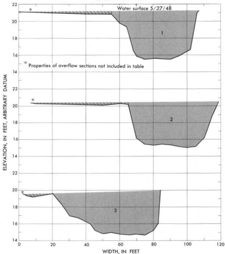
Plan sketch and cross sections, Catherine Creek near Union, Oreg.
