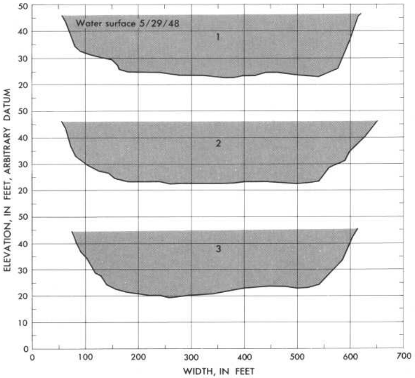
Plan sketch and cross sections, Clearwater River at Kamiah, Idaho.
