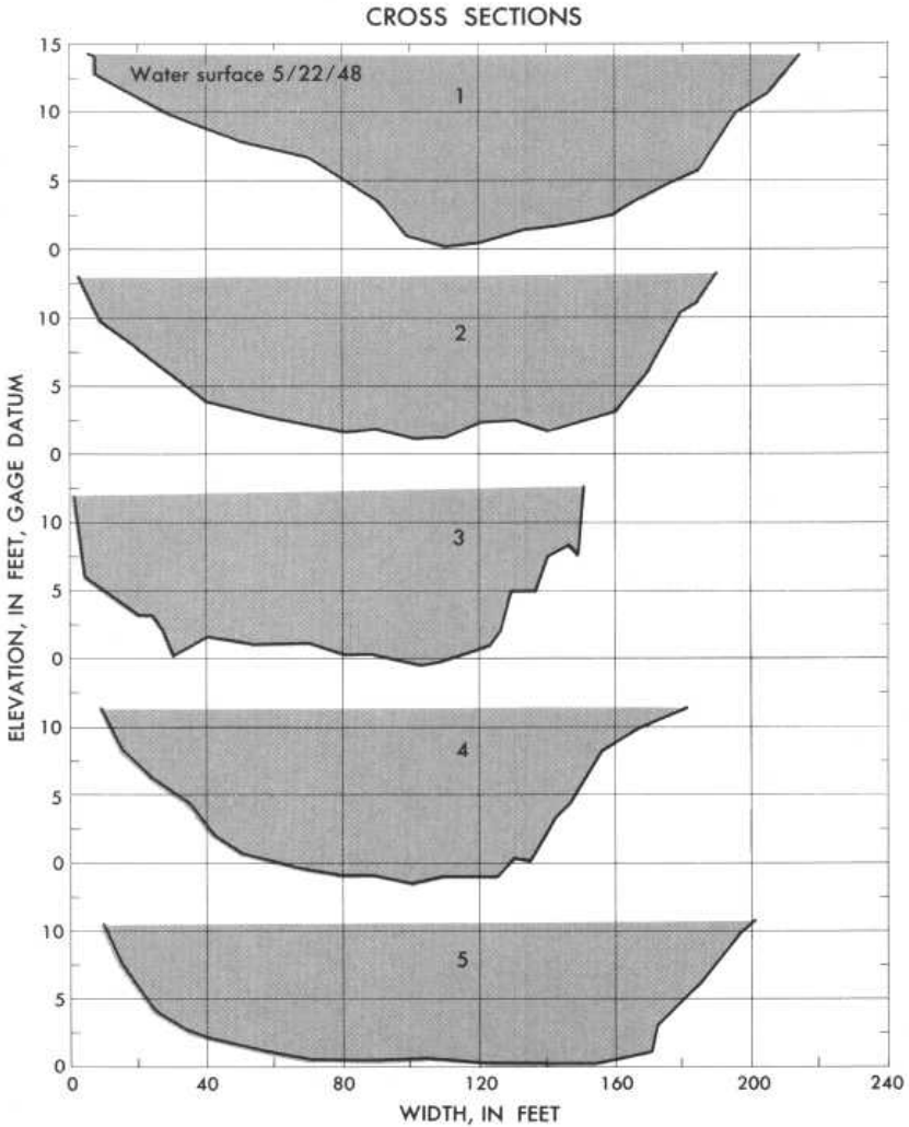
Plan sketch and cross sections, Middle Fork Flathead River near Essex, Mont.
