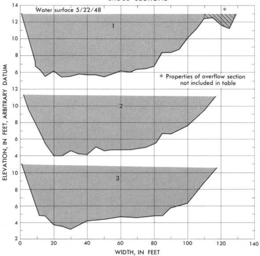
Plan sketch and cross sections, Grande Ronde River at La Grande, Oreg.
