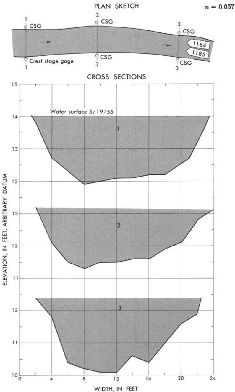
Plan sketch and cross sections, Mission Creek near Cashmere, Wash.
