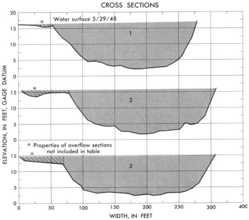
Plan sketch and cross sections, Wenatchee River at Plain, Wash.
