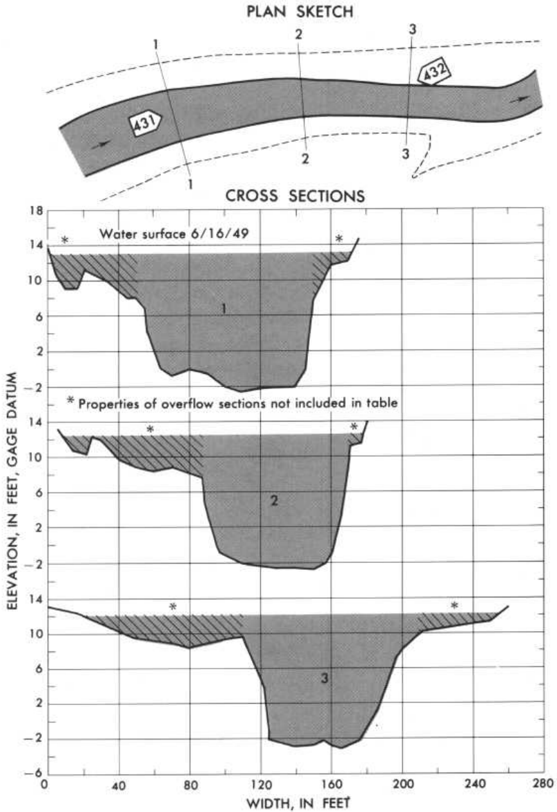
Plan sketch and cross sections, Hominy Creek at Candler, N.C. Dashed lines show limits of overbank flooding.
