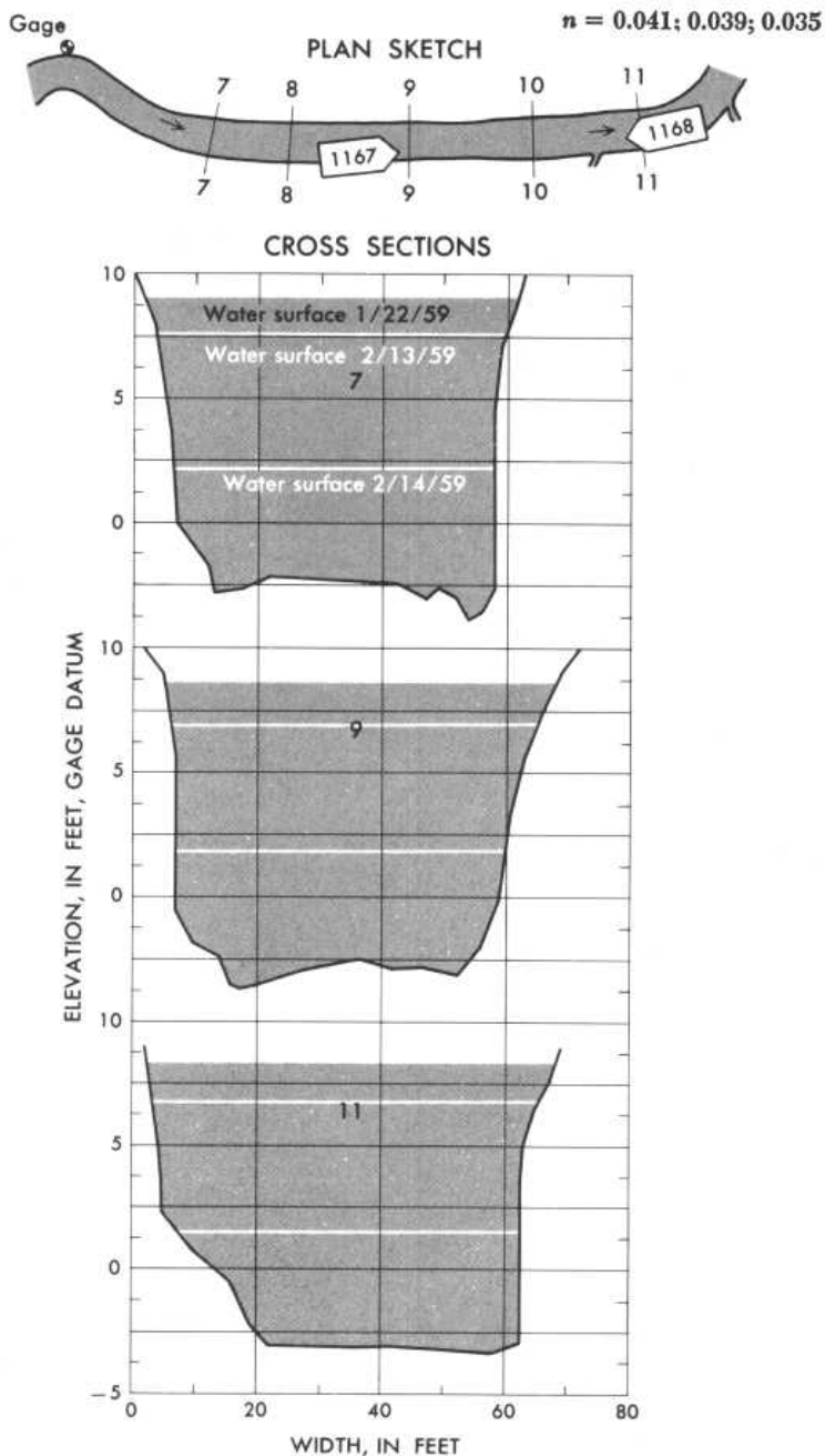
Plan sketch and cross sections, Etowah River near Dawsonville, Ga.
