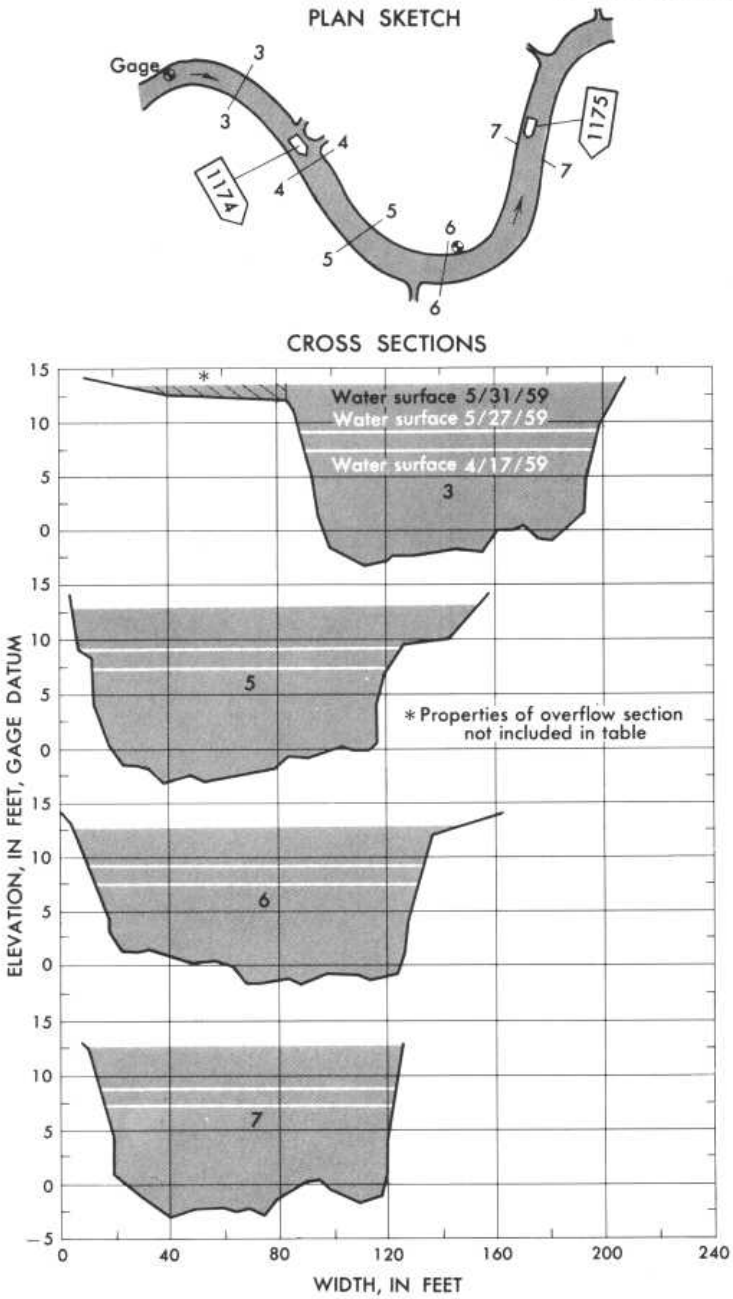
Plan sketch and cross sections, Middle Oconee River near Athens, Ga.
