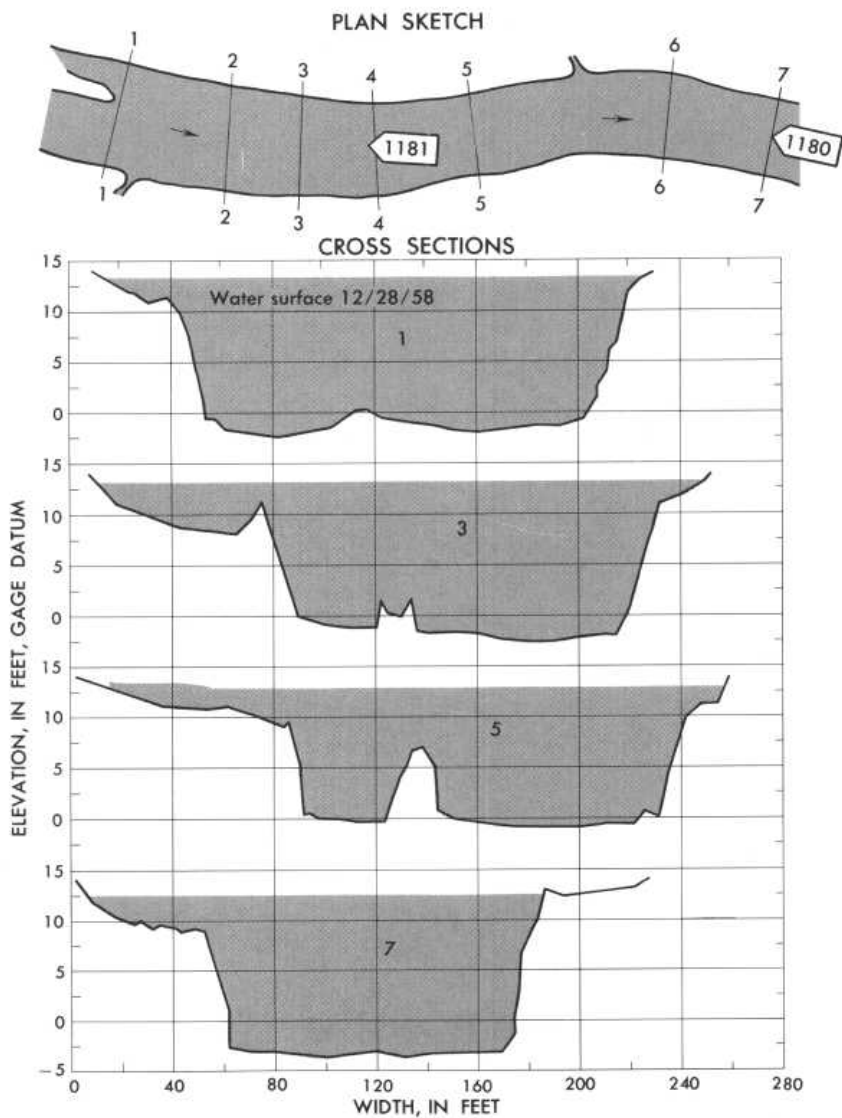
Plan sketch and cross sections, Deep River at Ramseur, N.C.
