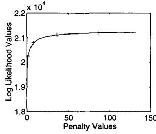
Fig. 4. Tradeoff curve for penalized estimation. This curve plots log likelihood versus penalty values as the weight \alpha varies. Each point on the curve is equivalently obtained by maximizing likelihood subject to a maximum value for the penalty. The "+" marks on the curve correspond to the images in Fig. 3.
