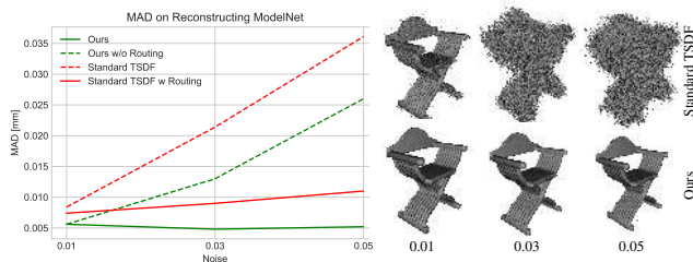
Figure 5: Evaluation of different noise levels \sigma . The left plot shows MAD for different noise levels \sigma \in \{0.01, 0.03, 0.05\} . Our routing network stabilizes both, our method as well as standard TSDF fusion, for high noise levels. On the right, we show corresponding qualitative results on ModelNet test data for Standard TSDF and our method. The figures show the denoising capability of our method, where standard TSDF fusion completely fails.
